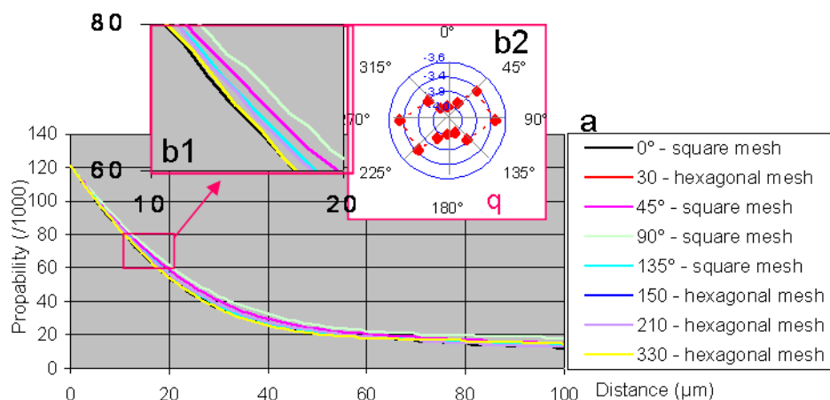
Fig. 13: a. Covariance curves in eight directions \alpha for alterite sample. It should be notice that 0° is vertical, perpendicular to the stratification. b1: Zoom on the slope at the origin ( N_L(X) ). b2: Slope ( q ) at the origin according to the direction \alpha
