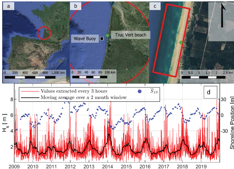
Figure 1. (a) Overview of the area (b) Location map of Truc Vert beach, southwest France indicating the position of the CANDHIS wave buoy (Cap Ferret wave buoy 03302). (c) Survey zone at Truc Vert beach. (d) Offshore wave height extracted at the location of the buoy for the considered period. The alongshore averaged in-situ shoreline is depicted in blue dots on the right axis.
