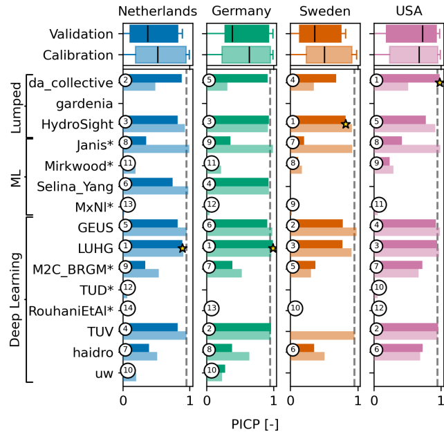
Figure 6. Bar plot of the PICP as a measure of the quality of the prediction intervals (0.95 is best, indicated by the vertical dashed line). The star in the bar plot indicates the best model. A star behind the team name indicates that the team provided confidence intervals instead of prediction intervals.
