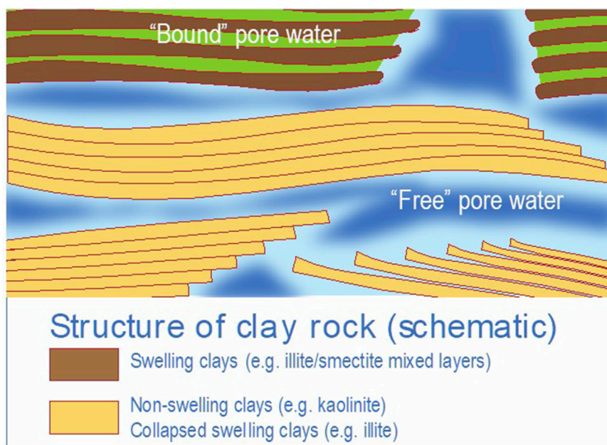
FIGURE 3 Texture of a clay rock, illustrating the various water properties and the heterogeneity of the different types of clay minerals at the nanometer scale. Dark blue colors indicate water domains with bulk water properties, light blue colors indicate water domains, which are influenced by the negatively charged surfaces of clay minerals and their electrical double layers (EDLs). Depending on the amount of fixed charges of the latter, the overall charge equivalents of positively and negatively charged solutes may vary within the different water domains. The green color represents water domains in the interlayers of swelling clays. Of note, the fractional distribution of clay and water domains does not represent the reality.
