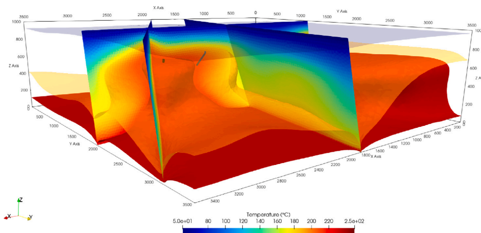
Fig. 5. Isotherm surfaces of 50 °C, 190 °C and 250 °C at the initial state, dominated by convection.
