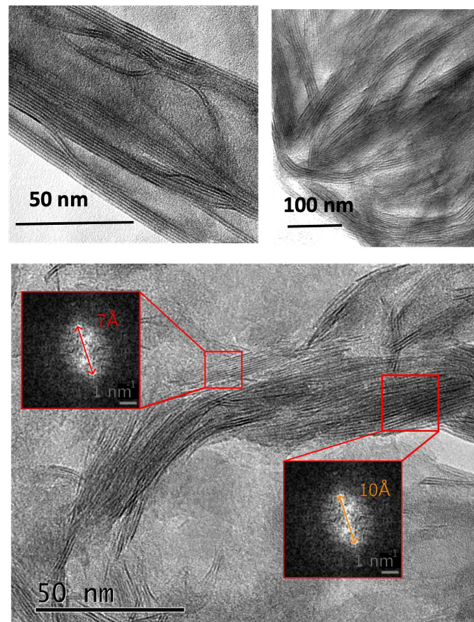
Figure 11. Main Ni-bearing mineral phase in ores from stage 1 to 3 observed under HR-TEM: talc-like from the blueish-green veins from stage 1; talc-like from pimelite ores in karst breccia (ore type 2); talc-like from ore type 3 (ferruginous saprolite). The talc-like are again found within the original serpentine framework inherited from the obduction stage. The talc-like are crystallised onto the serpentine layers at the nanometric scale.
