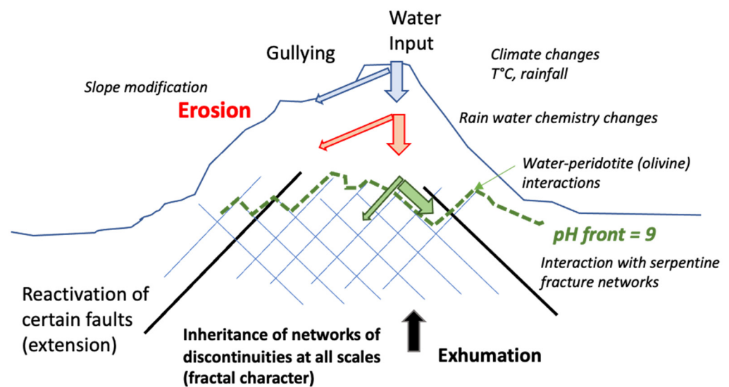
Figure 1. Main parameters controlling the weathering front development and deepening in the context of supergene alteration of peridotites.
