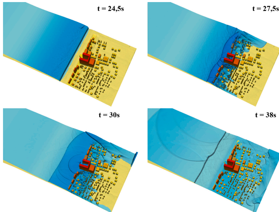
Fig. 17. Seaside : 3D view snapshots of the flooding evolution for increasing times of the simulation.
