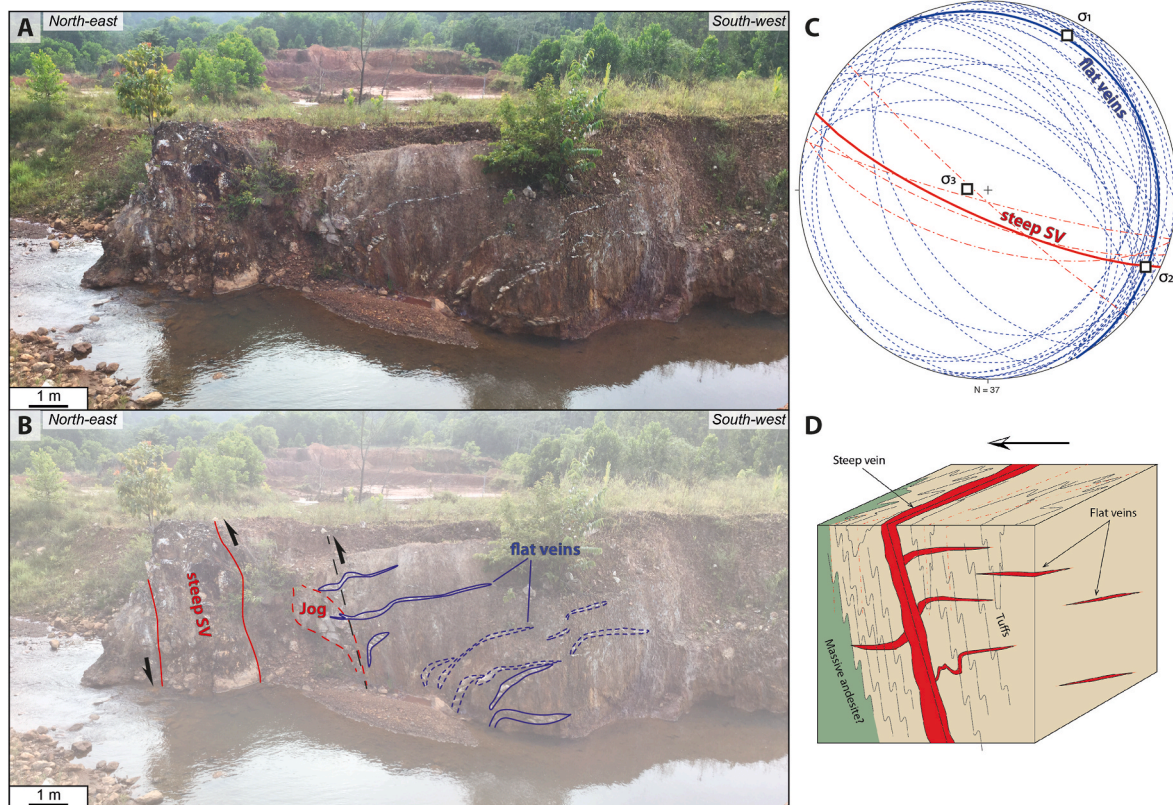
Fig. 7. Example of D_1 quartz-tourmaline vein system observed within Boulanger prospect. A and B. Field picture and interpretation showing the geometry of D_1 mineralized system. Note the presence of sub-horizontal (flat; blue) veins connected to steeply southwest dipping massive shear vein (red). C. stereographic projection of both shear (red) and extension (blue) veins. D. Block diagram showing the geometry of the D_1 -mineralized system.
