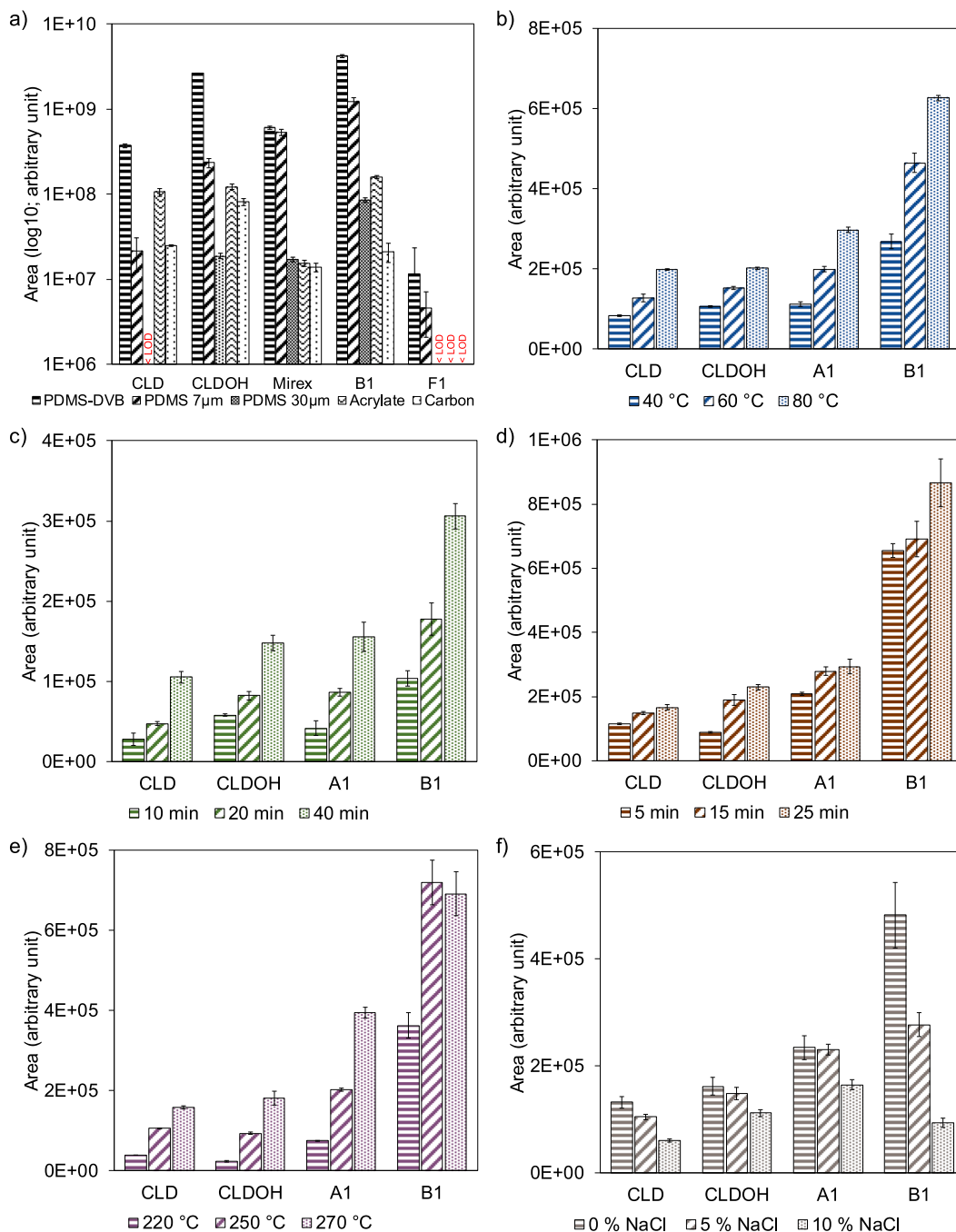
Fig. 3. Responses in SPME-GC-SIM/MS for CLD and its derivatives depending on: a) the SPME coating fiber (all concentrations set at 100 µg/L), b) the extraction temperature (all concentrations set at 1 µg/L), c) the extraction time (all concentrations set at 1 µg/L), d) the desorption time (all concentrations set at 1 µg/L), e) the desorption temperature (all concentrations set at 1 µg/L) and f) the addition of NaCl (all concentrations set at 1 µg/L). Error bars refer to standard errors (n = 3), <LOD: not detected.
