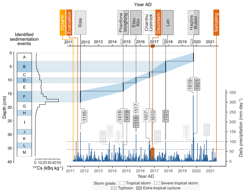
Fig. 4. (a) Identification of extreme precipitation events-associated deposits and (b) dating of these identified deposits by comparing 137 Cs distribution along the sediment core, progress of decontamination, and the extreme precipitation events that occurred since the Fukushima Daiichi Nuclear Power Plant (FDNPP) accident in March 2011. Decontam. stands for decontamination. Extreme precipitation events ranked as extra-tropical cyclone (solid), typhoon (dash), severe tropical storm (dot-dash) and tropical storm (dot) that generated more than 60 mm of daily precipitation (horizontal dotted line, Evrard et al. (2014)) are identified by their international number ID and named when associated with a deposit.
