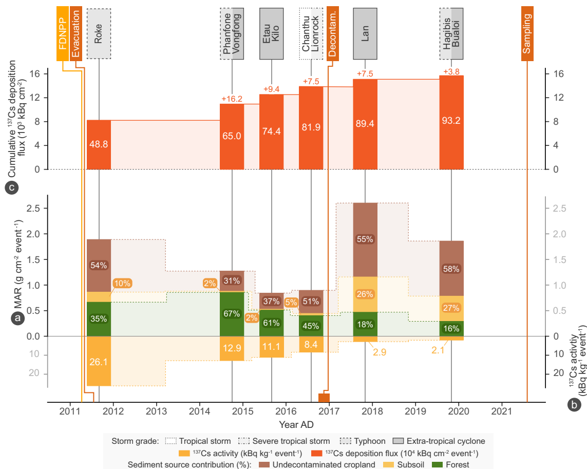
Fig. 8. Evolution of the (a) mass accumulation rate (MAR) as a function of the contribution of each sedimentary source (%), ^{137}\text{Cs} (b) activity and (c) cumulative deposition flux per extreme precipitation event identified along the sediment core sampled in the downstream part of the Mano Dam reservoir.
