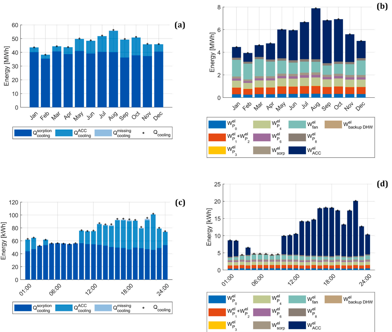
Fig. 9. Cooling sources and electricity consumption (a, b) on a monthly basis and (c, d) on an hourly basis for the 2nd of September 2050. Preliminary sizing defined in Table 2.
