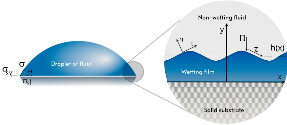
Fig. 1. 2D sketch of the thin wetting film sandwiched in between the solid substrate and the non-wetting fluid. Both inter-molecular interactions and fluid flow exert an excess stress – with a normal ( \Pi ) and a tangential ( \tau ) component – on the fluid-fluid interface. The inter-molecular interaction in the film can be expressed as a normal stress on the boundary of the film.
