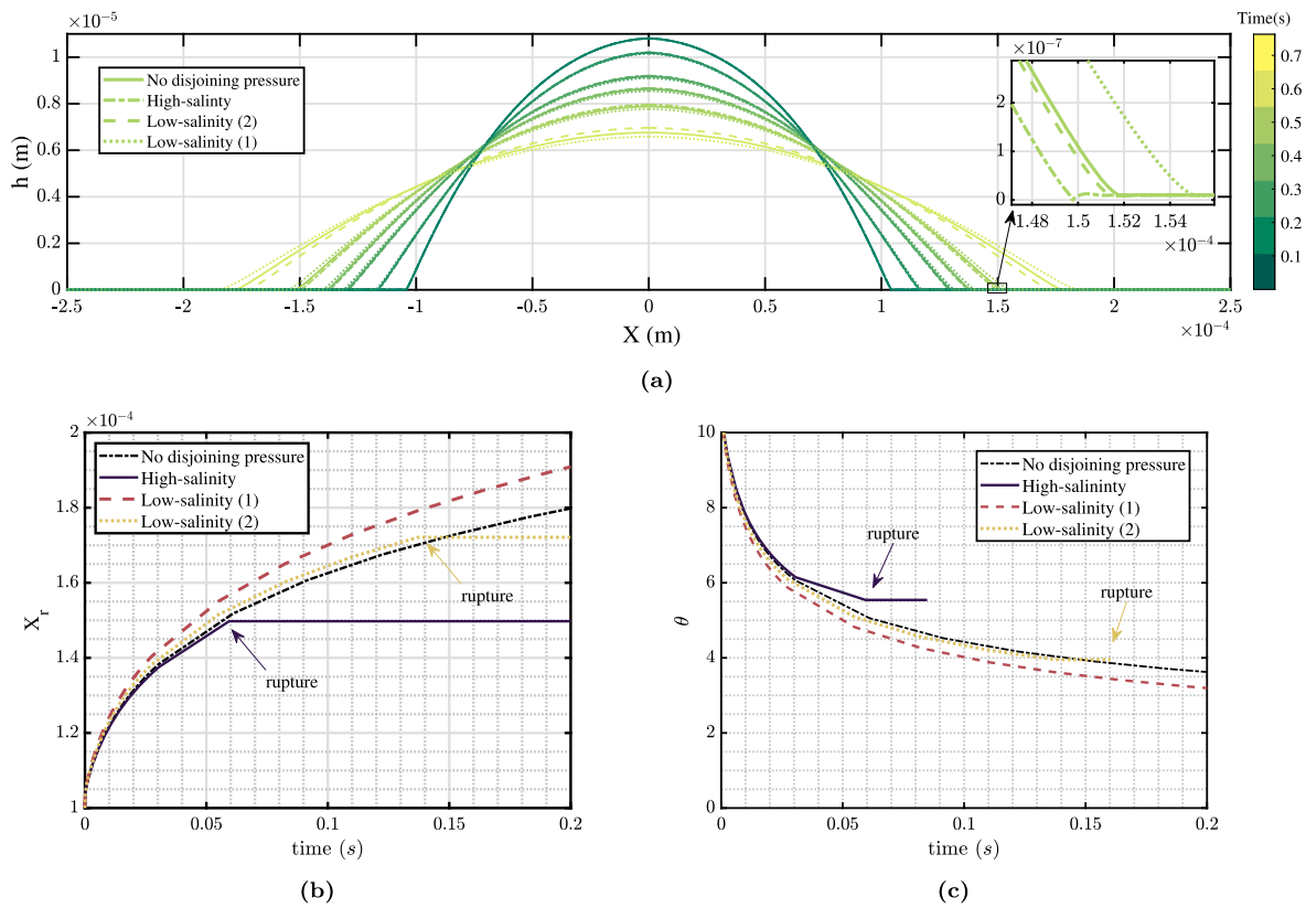
Fig. 7. Spreading of water in the system of water/oil/carbonate considering curvature, gravity, and disjoining pressure with the Bond number of 0.0166. (a) The plot of the water droplet profile for three different water types. Time is indicated by the color bar. In the inset plot, the profile of the film close to TPCP is shown at the time of rupture for high-salinity. The high-salinity water advances slower in comparison with the low-salinity cases and undergoes a rupture eventually. The transition of low-salinity (1) water to the precursor thickness occurs more smoothly compared to the high-salinity case. (b) Evolution of droplet radius. The spreading of high-salinity and low-salinity (2) water is halted at around 0.05 and 0.15 seconds, respectively, due to thinning of the precursor film at TPCP. (c) Variation of the contact angle at the inflection point with respect to time.
