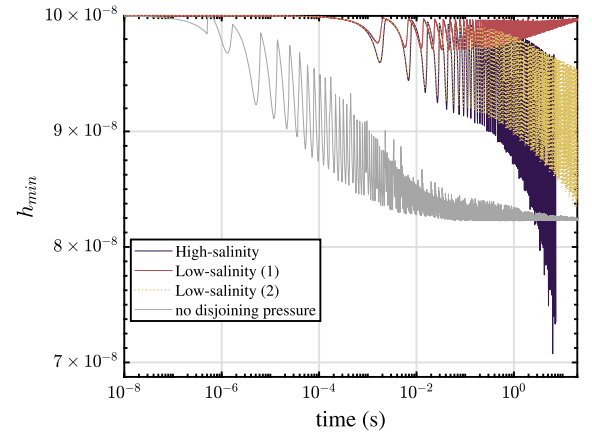
Fig. 9. The oscillation of TPCP thickness versus time for spreading of water with different properties. The oscillation in the case of low-salinity (1) gets dampened in late times, whereas for high-salinity, it grows until the rupture of the film. For low-salinity (2), the growth of amplitude of oscillation becomes steady in late times.
