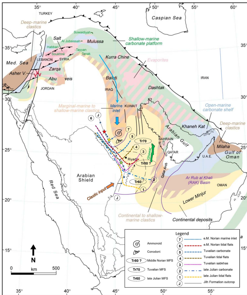
Figure 13. Extent of the main sedimentary events of the Jilh Formation, from late Julian to Middle Norian in chronologic order, as in outcrop, and inferred under the early Norian–pre-Minjur unconformity. Base map modified after Ziegler [2001] by permission of GeoArabia, with contribution of Le Nindre et al. [1990a] for the outcrop. For legend of the Jilh outcrop, see Figure 1.
