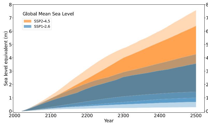
Figure 5. Projections of global mean sea-level rise to 2500 (m). Total global mean sea-level change to 2500 based on the projections in Figures 2–4. Combinations are made assuming full correlation. Darker shaded regions represent the 17%–83% intervals, and lighter shaded regions represent the 5%–95% intervals. Box and whiskers show the 17%–83% and 5%–95% intervals at 2500. All projections are relative to 2020.
