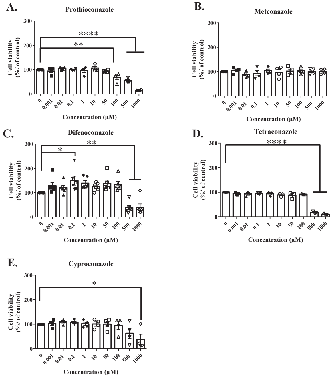
Fig. 3. Effect of triazoles exposure on human primary granulosa cell (hGCs) viability Dose effect (0.001–1000 \mu\text{M} ) of five triazoles (Prothioconazole (A), Metconazole (B), Difenoconazole (C), Tetraconazole (D) and Cyproconazole (E) for 24 h on cell viability of hGCs. Data are means \pm SEM of 3, 4 or 6 independent experiments. For one experiment of hGCs, a pool of cells from 3 patients was used for each triazole. The values were normalized with the control (without triazole exposure). Stars (*) correspond to the one-way ANOVA significance followed by the Dunnett's multiple comparison test or the Kruskal Wallis significance followed by the Dunn's multiple comparison corresponding to the comparison between control (without exposure) and the other triazole concentrations. *: p < 0.05 ; **: p < 0.01 ; ***: p < 0.001 ; ****: p < 0.0001 .
