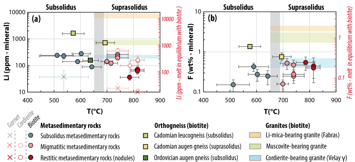
395 396 Fig. 6 Evolution of the average a Li and b F compositions of biotite, cordierite and garnet, with errors at 2 sigma 397 deviation (SD), as a function of peak temperatures for para- and ortho-derived metamorphic rocks from the Velay 398 dome. The range of Li-F contents in igneous biotite from Variscan granites is shown for comparison (colored 399 fields). Temperatures were calculated based on the Ti-in-biotite geothermometer (Henry et al. 2005) for subsolidus 400 metamorphic rocks and errors bars show 2SD. Mean temperatures and associated uncertainties for suprasolidus
