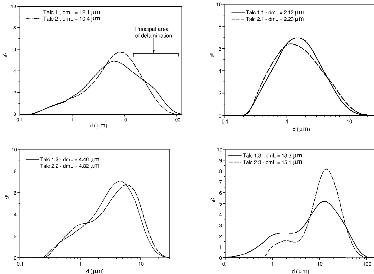
Fig. 4. Granulometric distribution of talc before and after delamination (talc 1 and 2, respectively), and aftergranulometric classification.
