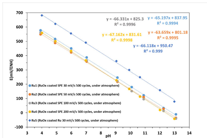
Figure 1: Open circuit potential of the RuO x electrode as a function of pH under oxic conditions.
