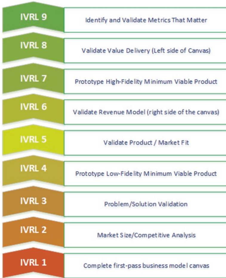
Fig. 1.5 IVRL levels
