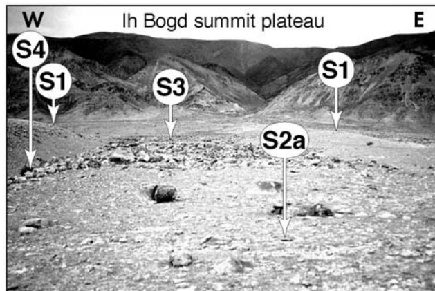
Figure 7. Surface S2 covered by the debris flow S3, which terminates upstream from the fault scarp.
