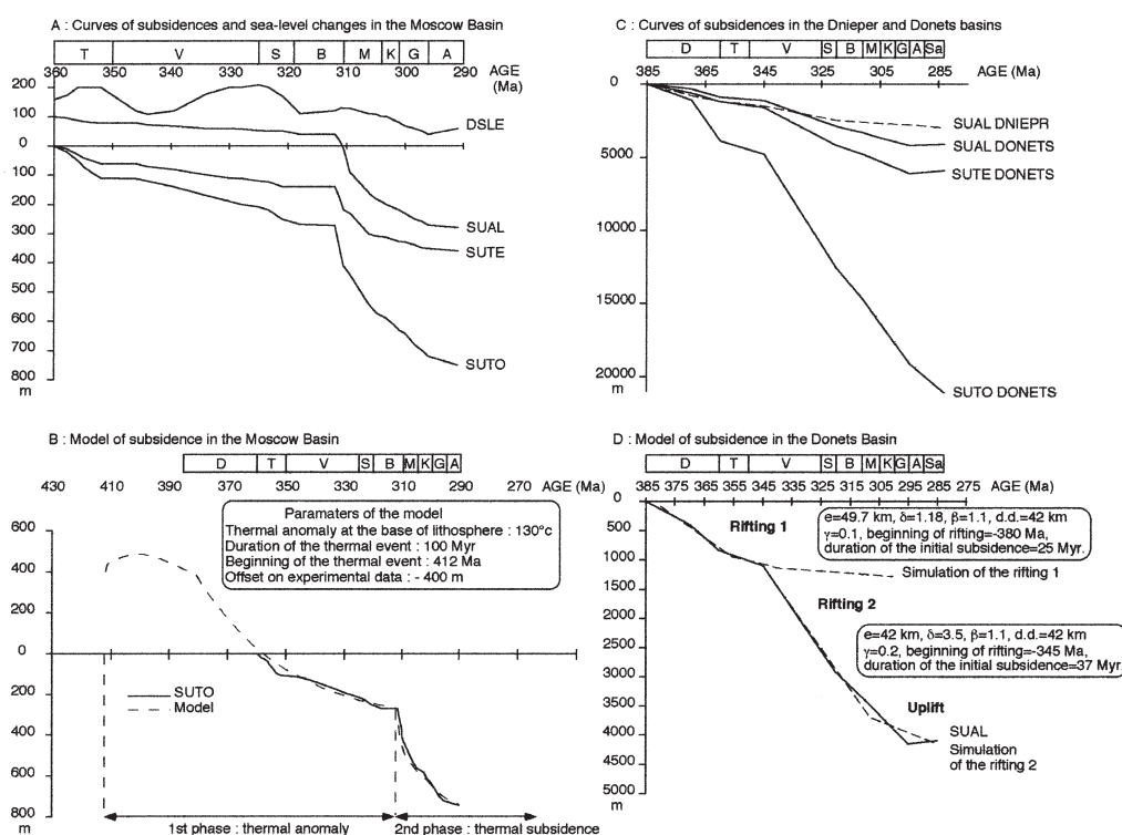
FIG. 3. — Curves of subsidences and models of subsidence in the Moscow and Dniepr-Donets basins.
