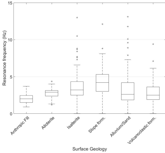
Figure 11. Distribution of the H/V peak values (dominant resonance frequency) regarding simplified surface geology given in Figure 1. For each box, the central line represents the median, the edges of the box represent the 25th and 75th percentiles, the whiskers (dotted lines) extend to 1.5 times the interquartile ranges, and the outliers (data with values beyond the ends of the whiskers) are plotted individually (crosses). Corresponding values are indicated in Table 4.
