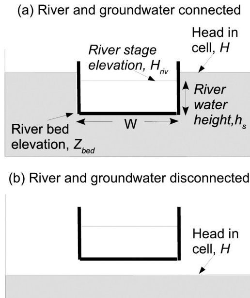
Figure A1. River-aquifer exchanges for (a) river and groundwater connected and (b) river and groundwater disconnected (Vergnes and Decharme 2012).
