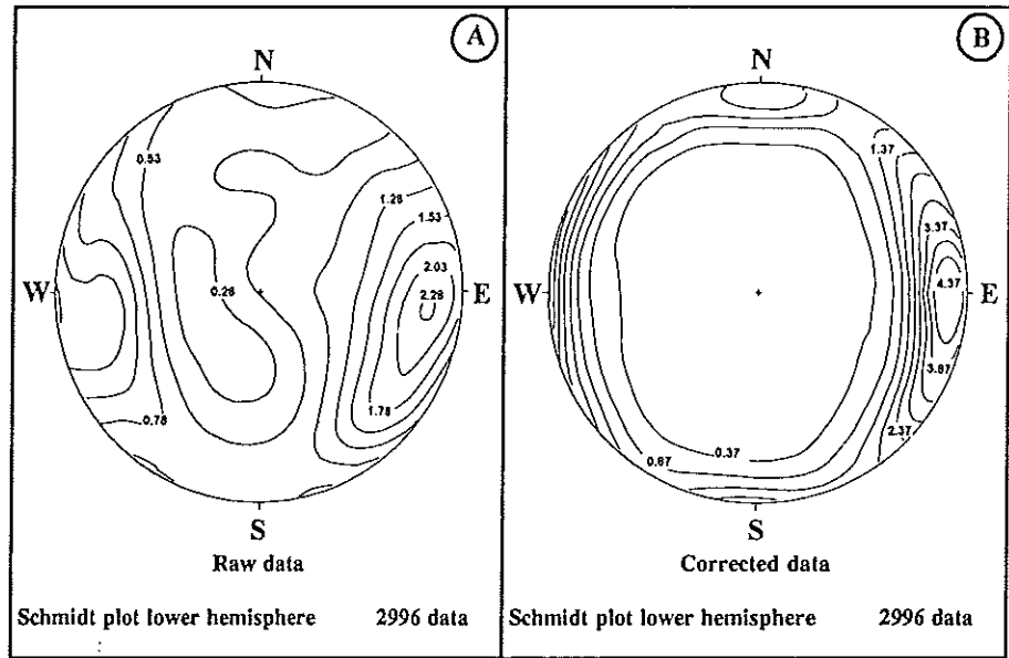
Figure 4 Lower-hemisphere density projections of natural fractures recorded on EPS-1 core sections (A) before and (B) after correction for borehole sampling bias according to the method of Terzaghi (1965).
