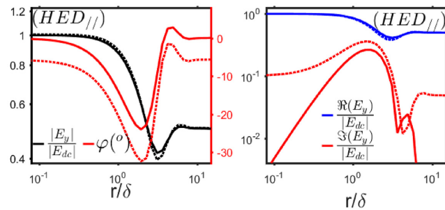
Figure 1. Normalized amplitude and phase (left-hand panel) and normalized in-phase and quadrature (right-hand panel) electric field responses for an inline HED, considering a 100 \Omega\cdot\text{m} real resistivity model with and without -100 mrad of CR phase delay. Dotted lines represent the CR model response whereas solid lines represent the real and constant resistivity response (without IP effect).
