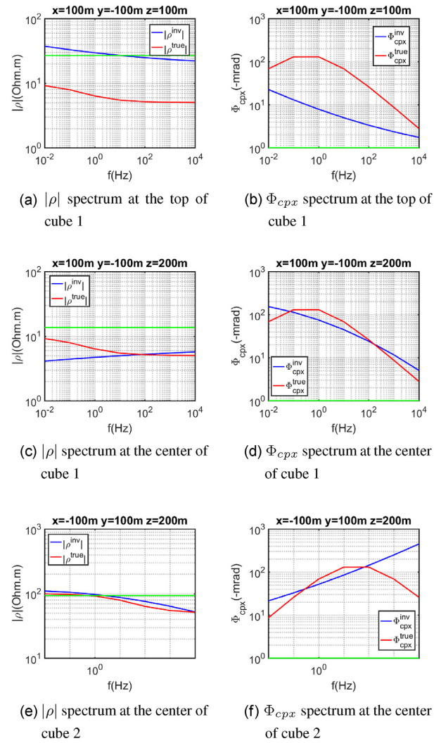
Figure 21. CR spectra at the centre of the cubes and at the top-centre of cube 1 for the two-cubes model. Green curves are the spectrum at the end of previous inversion stage (stage 0 for |\rho| and stage 1 for \Phi_{cpx} ).
