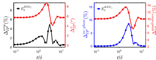
Figure 2. IP effect on amplitude and phase delay (left-hand panel) and on in-phase and out-of-phase (right-hand panel) electric fields on a 100 \Omega\cdot\text{m} real resistivity homogeneous half-space with -100 mrad of CR phase delay.
