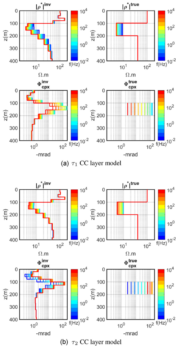
Figure 11. Inversion results for the \tau_1 and \tau_2 CC layer models with, respectively, a low and a high EM/IP coupling using a 500 m profile of 21 receivers and an inline HED source as described in Fig. 8. Note that |\rho^*|^{inv} subplot are the results of stage 1 and are not modified during stage 2, whereas subplot \phi_{cpx}^{inv} are the results of stage 2 and were kept at the starting model values during stage 1 as only |\rho^*| is inverted.
