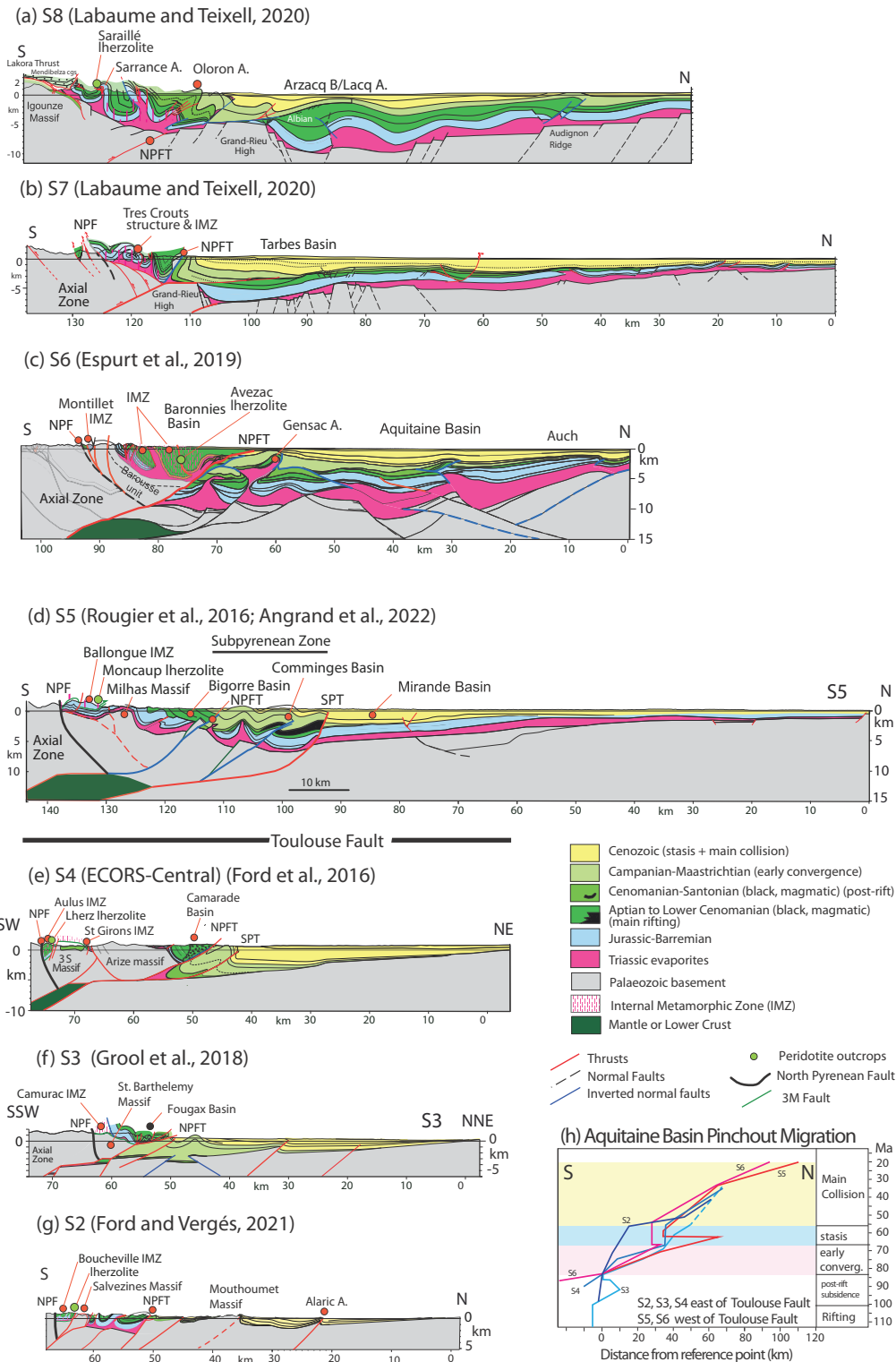
Fig. 7. Compilation of seven cross-sections across the Pyrenean retroforeland system from west to east and located on Figure 3 . Authors' estimates of retrowedge shortening are shown in brackets. Estimates derived from cross-section restoration are indicated with an R. Sections are simplified and adapted from (a) and (b) Labaume and Teixell (2020) and Jourdan et al. (1998) for northern basins (10–15 km), (c) Espurt et al. (2019a, b) (R ~ 42 km), (d) Rougier et al. (2016) and Angrand et al. (2022) (R ~ 12.5 km), (e) Ford et al. (2016) (R ~ 30 km), (f) Grool et al. (2018) (R ~ 19 km) and (g) Ford and Vergés (2021) (R ~ 10–12 km). Estimates of shortening exclude emplacement of the Internal Metamorphic Zone (IMZ) and closure of exhumed mantle domains. (h) Graph of pinchout migration of the northern margin of the Aquitaine basin on sections S2 to S6. Colored bars represent orogenic stages as in Figures 5b and 5c .
