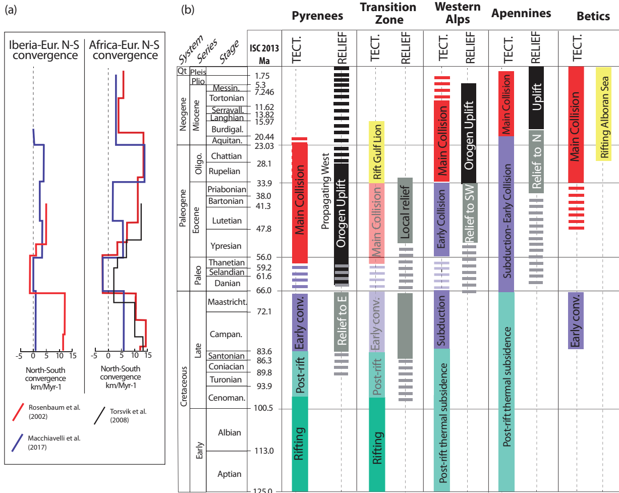
Fig. 2. Plate kinematics and distribution of deformation across the west Mediterranean. (a) North-south component of Iberia-Europe and Africa-Europe plate movement vectors from Rosenbaum et al. (2002a, b), Macchiavelli et al. (2017) and Torsvik et al. (2008). The vertical scale is the same time scale as in b. (b) Chronology of major tectonic events and evolution of orogenic relief around the western Mediterranean using the International Stratigraphic Chart (2013), IUGS. Data supporting the tectonic stages and relief of the Pyrenees and in the transition zone (Provence, Fig. 1) between the Pyrenees and Alps are presented in this paper. For the Alps see Le Breton et al. (2020) and references therein; for the Apennines see Marroni et al. (1992), Molli (2008) and Conti et al. (2020); for the Betics see Vergés and Fernández (2012).
