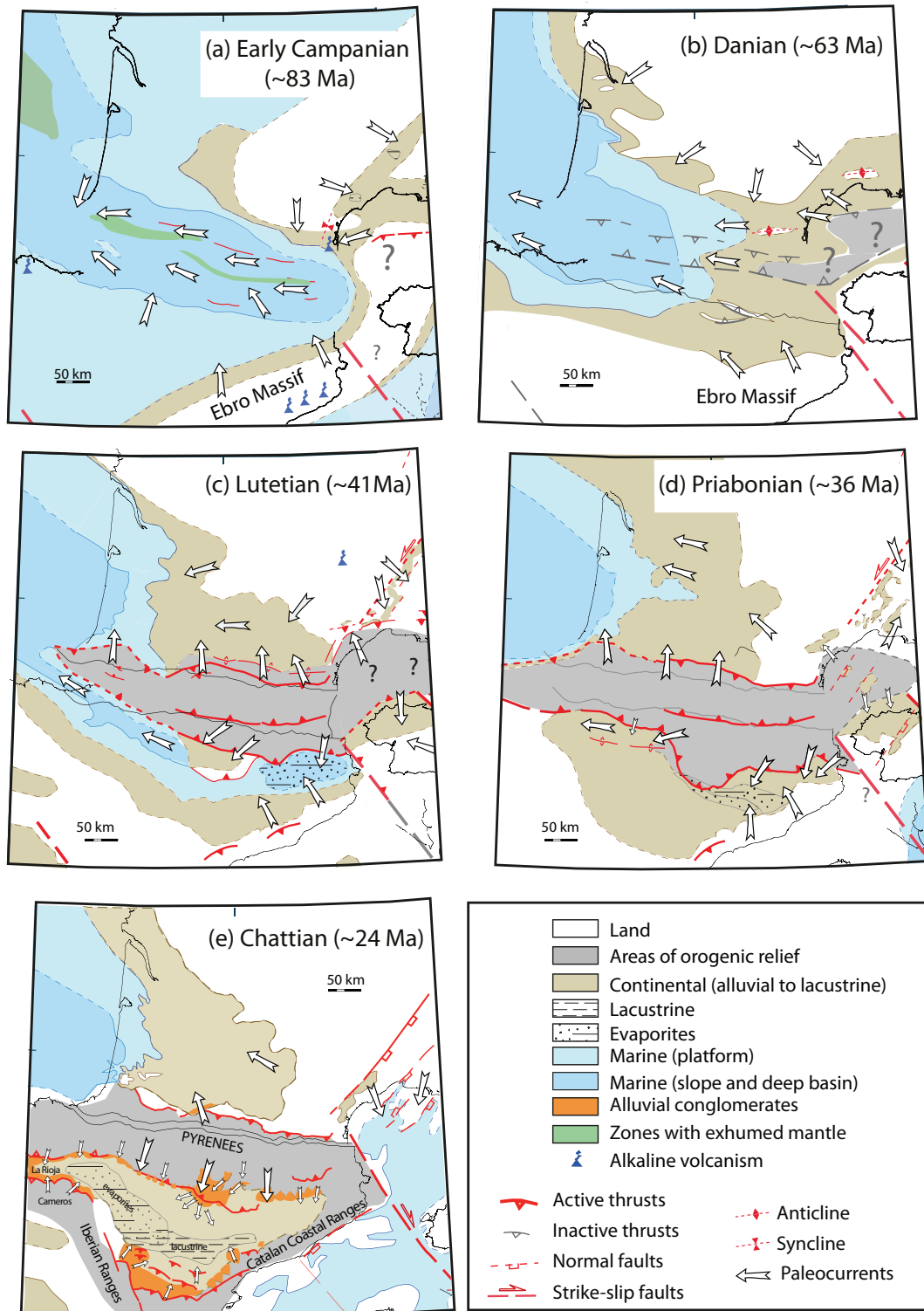
Fig. 6. Paleogeographic reconstructions of the evolution of Pyrenean synorogenic basins, orogenic relief and sediment supply from base Campanian to Oligocene. Using the free G-Plates 2.0 software (Müller et al. , 2018) present-day coastlines were restored back in time following the plate kinematic model of Macchiavelli et al. (2017) for the western Mediterranean. Paleoenvironments are based on Plaziat (1981), Debrand-Passard et al. (1984), Barnolas and Courbouleix (2001), Serrano et al. (2006) and Monod and Bourroullec (2014) with restorations by G. Frasca using balanced cross-section presented in Figures 7 and 8 and Vergés (1993). Deformation characteristics (timing, principal structures, amount of shortening) and basin evolution (basin limits, dynamics, major facies, paleocurrents) were integrated using published data. Uncertainties related to the plate kinematic model were reduced by assuring that each step honored data on vertical motion, structural and stratigraphic history.
