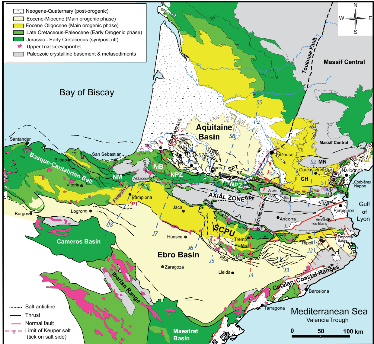
Fig. 3. Simplified geological map of Pyrenees. Abbreviations in northern Pyrenees: NPFT: North Pyrenean Frontal Thrust; NPZ: North Pyrenean Zone; NPF: North Pyrenean Fault; SZ: Subpyrenean Zone; MB: Mauléon Basin; CH: Carcassonne High; CLTZ: Corbières-Languedoc Transfer Zone. North Pyrenean basement massifs: AS: Agly-Salvezines; MM: Mouthoumet; MN: Montagne Noire Massif; BS: Saint Barthelemy; 3S: Trois Seigneurs. Abbreviations in southern Pyrenees: South Central Pyrenean Units; NT: Noguères Thrust; BT: Bóixols Thrust; MsT: Monsec Thrust; SMT: Serres Marginals Thrust; BBA: Barbastro-Balaguer Anticline; SA: Sanauja Anticline; TR: Transverse Ranges. Blue dashed lines locate cross-sections in Figures 7 and 8 and some crustal scale cross-sections along the same lines in Figure 4 . Red dashed lines ECORS deep seismic crustal cross-sections ( Fig. 4 ) and the deep seismic tomography profile P1 ( Chevrot et al., 2018 ) in the NW Pyrenees.
