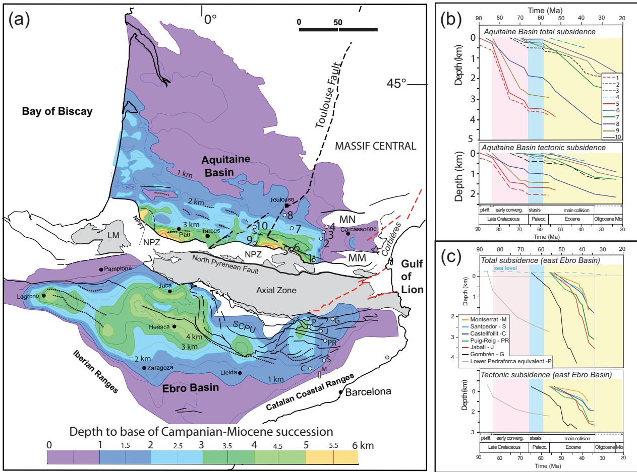
Fig. 5. (a) Present day isodepth map to base of syn-orogenic sediments in km in the onshore Ebro and Aquitaine basins compiled from Angrand et al. (2018) for the Aquitaine basin and Garcia-Castellanos et al. (2003) for the Ebro Basin. (b) Total and tectonic synorogenic subsidence curves for ten boreholes in the central and eastern Aquitaine basin. Boreholes are located in (a). Data compiled from Groot et al. (2018; 1–4) , Ford et al. (2016; 5–8) and Rougier et al. (2016, 9–10) where details of data and calculations can be found. (c) Total and tectonic synorogenic subsidence curves for seven boreholes in the eastern Ebro basin (for details see Groot et al. , 2018 ). Boreholes and stratigraphic logs used in these calculations are located in (a). The orogenic stages of early convergence, quiescence (stasis) and main collision are indicated by colored bands on the graphs. For abbreviations see Figure 3 caption.
