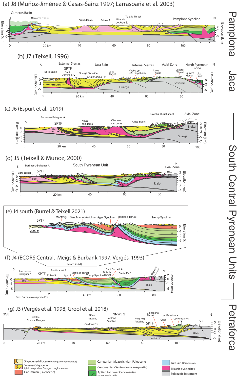
Fig. 8. Cross-sections across the south Pyrenean foreland system, all located in Figure 3 and organised from west to east. Shortening estimates across the whole south vergent system of cited authors, derived from cross-section restoration, are shown in brackets. (a) J8 (~ 40 km) adapted from Larrasoña et al. (2003) and Muñoz-Jiménez and Casas-Sainz (1997) ; (b) J7 (48 km), adapted from Teixell (1996) . (c) J6 (85 km) adapted from Espurt et al. (2019a, b) . (d) J5 (> 60 km) adapted from Saura et al. (2016) . (e) Detailed section along the southern South Central Pyrenean Unit of the ECORS central line (J4 south, Fig. 3 ) showing strong salt influence, adapted from Burrell and Teixell (2021) . (f) J4 (66–88 km) along the ECORS central deep seismic line adapted from Meigs and Burbank (1997) and Vergés (1993) . (g) J3 (92 km) adapted from Vergés et al. (1998) and Grool et al. (2018) .
