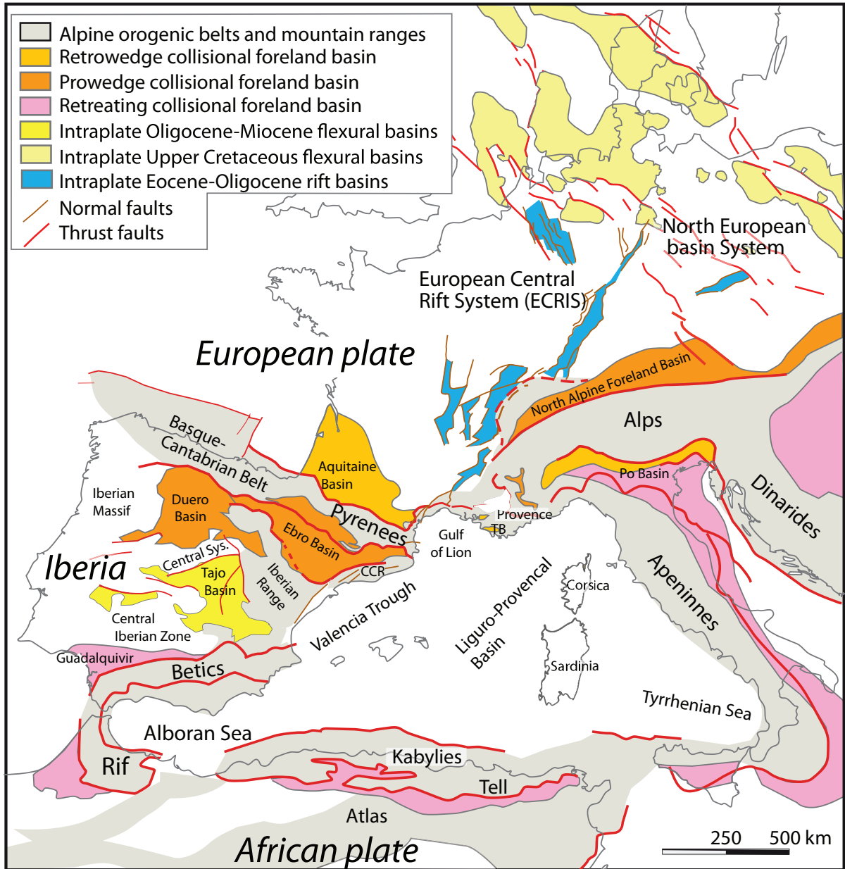
Fig. 1. West Mediterranean and western Europe alpine orogens, and onshore synorogenic basins (Late Cretaceous-Cenozoic). Abbreviations: TB: Toulon Belt, Provence; CCR: Catalan Coastal Ranges.
