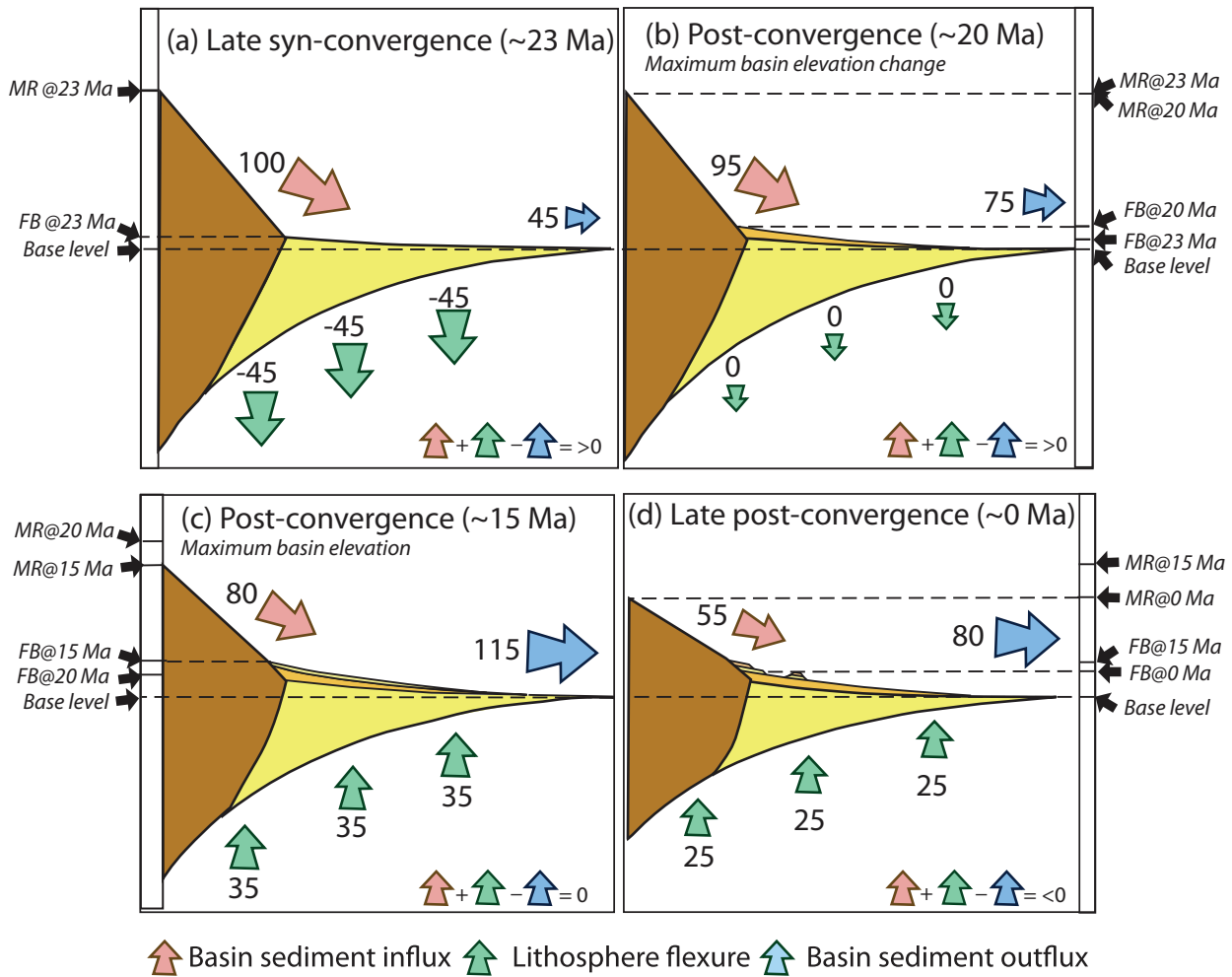
Fig. 11. Schematic representation of results of numerical modelling of Bernard et al. (2020) simulating the transition from syn-convergence to post-convergence in four time frames, designed to represent the sedimentation and erosion record along the North Pyrenean thrust front from early Miocene to present day. Red, green and blue arrows correspond respectively to three controlling parameters, the basin influx from the orogen, lithospheric flexure (positive is uplift, negative is subsidence) and basin outflux. Numbers next to arrows indicate a percentage contribution to the basin elevation based on model results detailed in Bernard et al. (2020). The sum of these values (see inset on each cartoon) results in an increase in elevation of the foreland basin in (a) and (b), stasis in (c), and erosion leading to a decrease in elevation in (d). (a) Latest syn-orogenesis at ~ 23 Ma (end of plate convergence). (b) Early post-orogenesis at ~ 20 Ma when positive elevation change of the foreland basin is maximum. (c) Post-orogenesis at ~ 15 Ma when elevation of the foreland basin is maximum. (d) Post-orogenesis at ~ 0 Ma when elevation of both the range and foreland basin are decreasing. Black arrows indicate elevation of the mountain range (MR) and foreland basin (FB) for the specific time frame and for the previous step for comparison. Adapted from Bernard et al. (2020).
