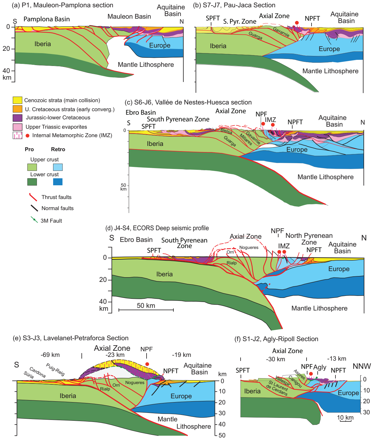
Fig. 4. Published crustal scale cross-sectional models across the Pyrenees from west to east, located in Figure 3. Authors estimated total shortening across the orogen is shown in brackets. (a) Interpretation of the deep seismic tomography model of Wang et al. (2016) along P1 adapted from Saspiturry et al. (2020) and Lehujeur et al. (2021). These authors do not provide a shortening estimate and do not distinguish upper and lower crust. (b) J7-S8 adapted from Teixell et al. (2016) (114 km). (c) J6-S6 adapted from Espurt et al. (2019a) (127 km). (d) J4-S4 (ECORS central deep seismic line) based on Muñoz (1992) and redrawn from Mencos et al. (2015) (147 km). (e) J3-S3 simplified from Grool et al. (2018) (> 111 km, distribution shown). (f) J2-S2 adapted from Ternois et al. (2019a, b) (43 km, distribution shown). Abbreviations: SPFT: South Pyrenean Frontal Thrust; NPFT: North Pyrenean Frontal Thrust; NPF: North Pyrenean Fault; IMZ: Internal Metamorphic Zone. The 3M Fault is identified on sections d, e and f.
