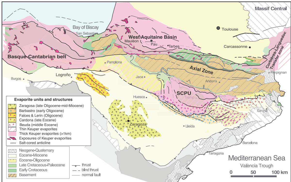
Fig. 9. Simplified tectonic map of the Pyrenees and adjacent regions (adapted from Vergés et al. , 2002) showing the distribution of evaporitic deposits of Upper Triassic and Cenozoic age. Based on Caméra (2017) and Caméra and Flinch (2017) for the Basque-Cantabrian belt and South Central Pyrenean Unit. In both the western Aquitaine Basin-Mauléon and the Corbières-Languedoc Transfer Zone evaporite distribution is mostly compiled from French BRGM geological maps, with data from Curnelle et al. (1982), Viillard (1987), Gorini et al. (1991) and Serrano et al. (2006) and Crémades et al. (2021). The distribution of Eocene to early Miocene marine and lacustrine evaporites in the Ebro Basin is based on Vergés (1993) in the east and Garcés et al. (2020) in the west.
