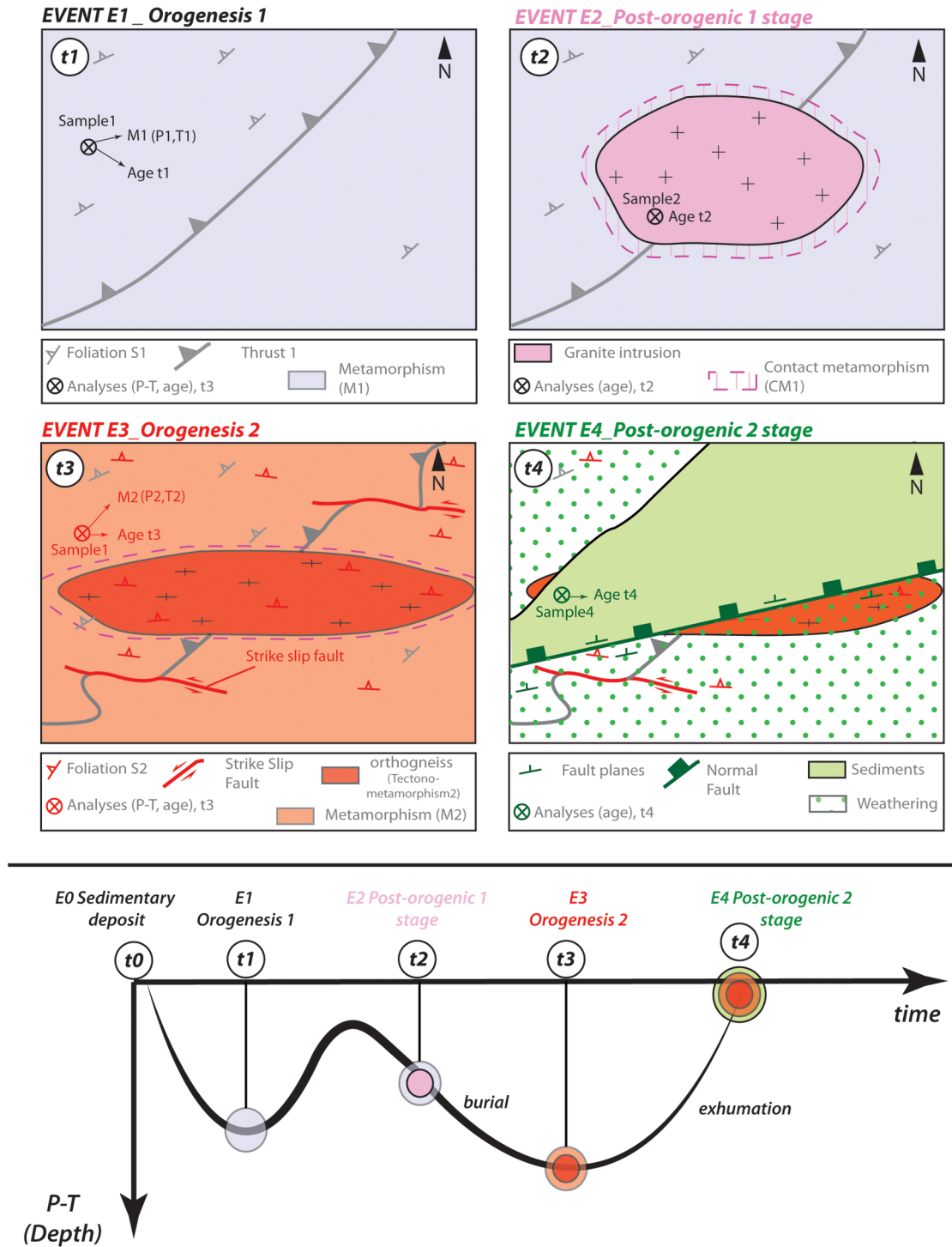
Fig. 10. Schematic successive geological-event maps corresponding to different geological stages. Polygons (geological units), polylines (faults, fold axes, metamorphic isograds, etc.) and points (measurements, analyses, etc.) are linked to different geological events capitalized in the geological-event reference system. All types of mapped features can be linked to a same geological event. This new method makes it possible to provide different digital maps through time.
