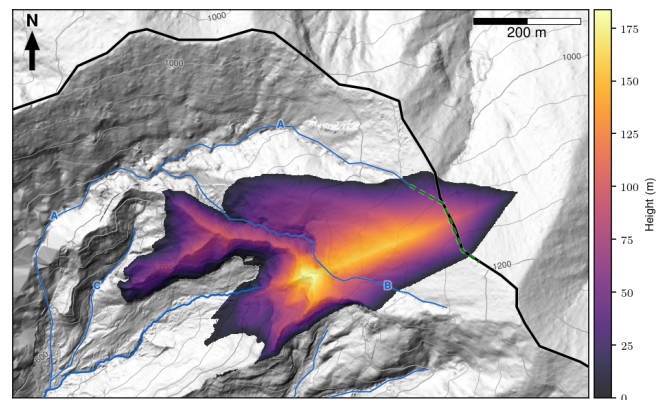
Figure 8. Potentially unstable volume. The height between the reconstructed basal surface (see Fig. 7b) and the combined July 2010–August 2018 DEM (displayed here) is given by the color scale. We only display heights above the contact between D and UPd units, as well as LPd and Upd units, and disregard heights below 1 m. The Samperre river (thick blue line), ravines (thin blue lines) and the Prêcheur destabilization structure (black line) are displayed as in Fig. 1. The unstable volume is computed either directly or by limiting the extent of the collapse (i) to ravine A continued along a topographic edge (dashed green line) or (ii) to ravine B (see Table 3).
