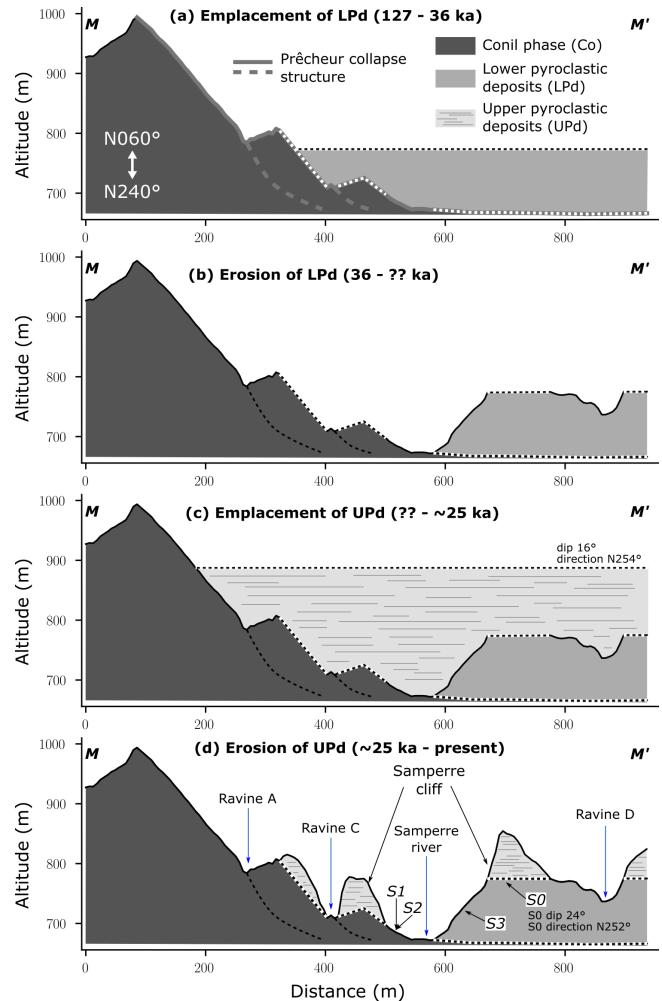
Figure 6. Conceptual view of the evolution of the paleo-morphology of the Samperre cliff, along a northwest (left) to southeast (right) cross-section (MM' in Fig. 1b). The figure is facing the northeast direction (60° N). (a) Emplacement of unit LPd within the Prêcheur collapse scar. The horizontal lines display deposition horizons, whose dip and dip direction are indicated. (b) Erosion of unit LPd, resulting in a paleo-valley at the location of the actual Samperre cliff. (c) Emplacement of unit UPd. (d) Erosion of unit UPd, resulting in the formation of the Samperre cliff and adjacent ravines. Black lines correspond to the topography given by the August 2018 DEM. Dashed white lines are interpretations of old topographies and contact between geological units. See Fig. 1c for the position of ravines.
