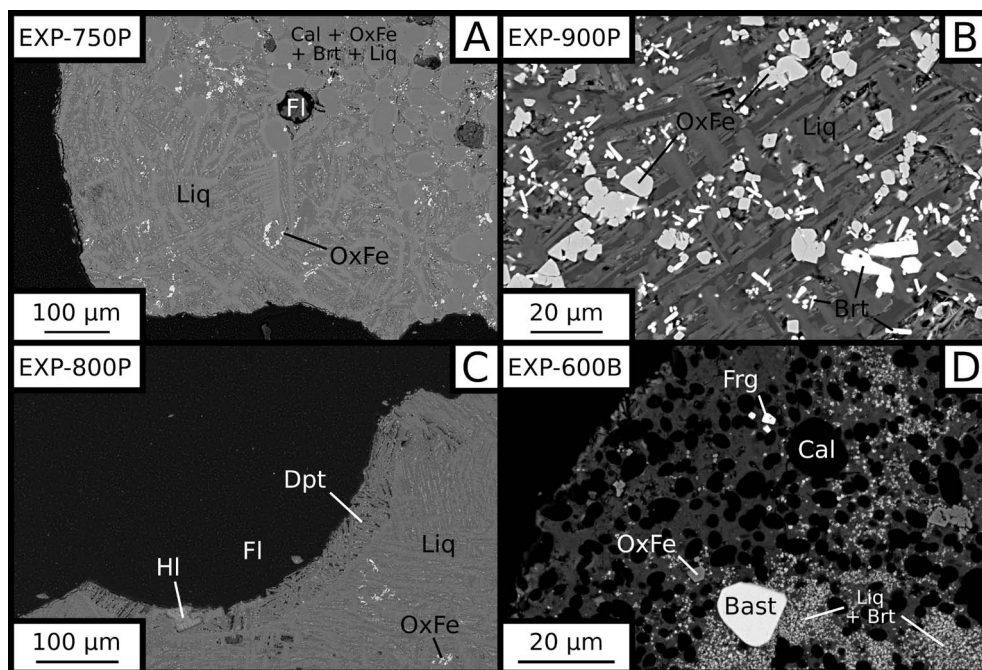
Figure 1. BSE images of samples. (A) melt and segregated calcite, iron oxides and britholite. (B) Euhedral britholites and iron oxides. (C) Vesicle filling hosting anhydrous halite inside a vesicle. (D) Bastnaesite and fergusonite in the saturation experiment. Liq: carbonate melt. Cal: calcite. OxFe: iron oxide. FI: vesicle (fluid indicator). Dpt: deposit-like vesicle filling. HI: halite. Brt: britholite. Bast: bastnaesite. Frg: fergusonite.
