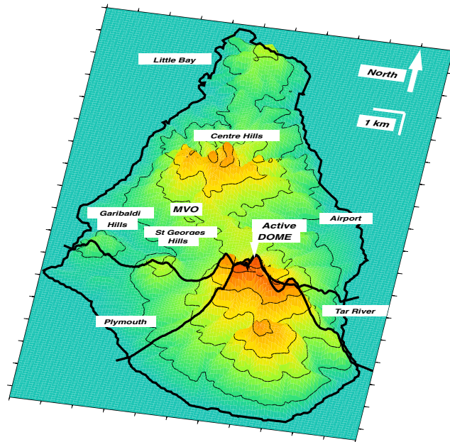
Figure 14. 3-D topographical map of Montserrat island, revealing the steep slopes of the volcano. The view is taken from the azimuth 170^\circ from N with an vertical view angle of 45^\circ . The black lines across the island indicate two topography profiles used to compute our synthetics.
