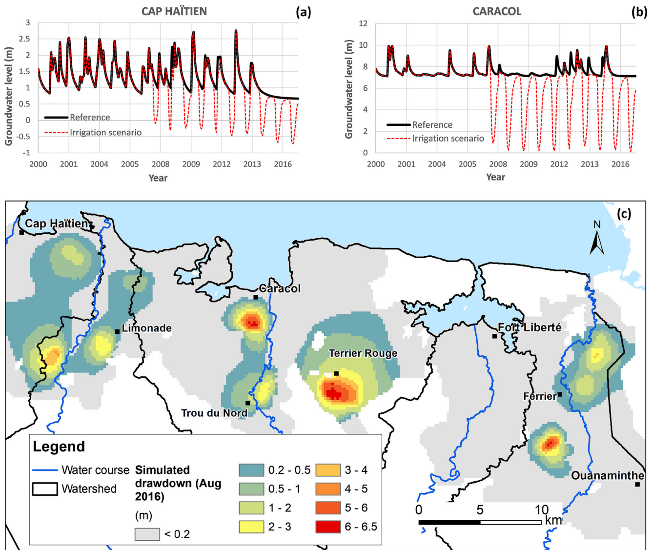
Fig. 16 Simulated drawdowns for the irrigation scenario (August 2016), with a variation of simulated heads in Cap-Haïtien area (for a 1-m diameter well), b variation of simulated heads in Caracol area (for a 1-m diameter well), and c simulated drawdown map
