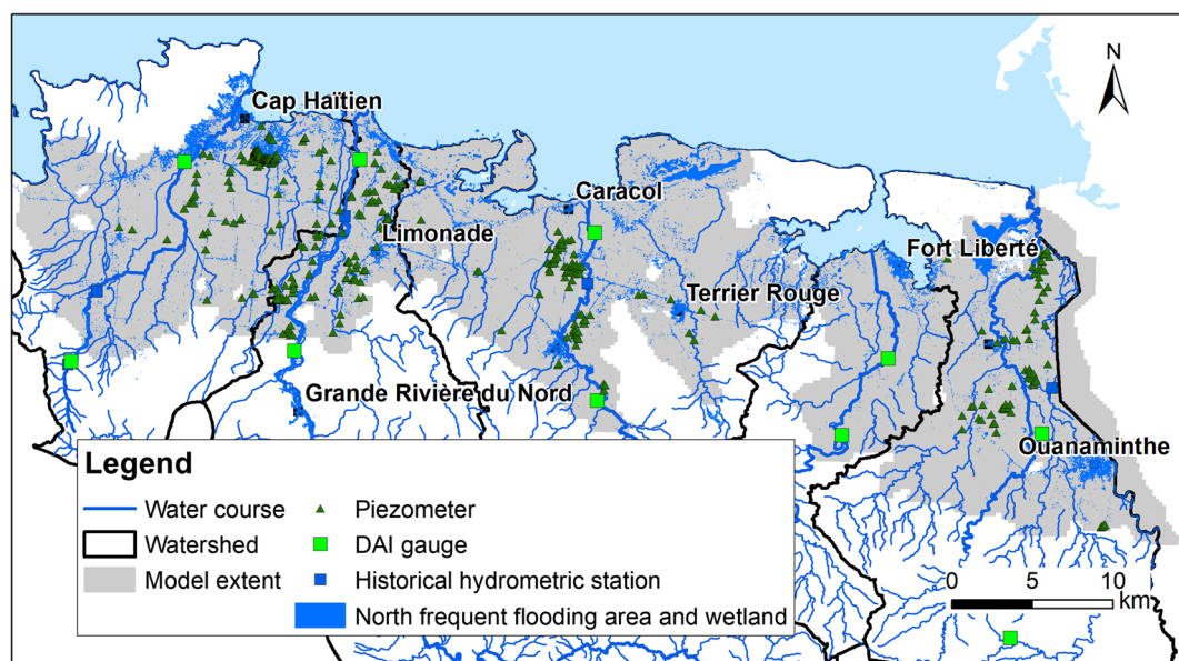
Fig. 8 Head and hydrometric data available for the steady-state model calibration
