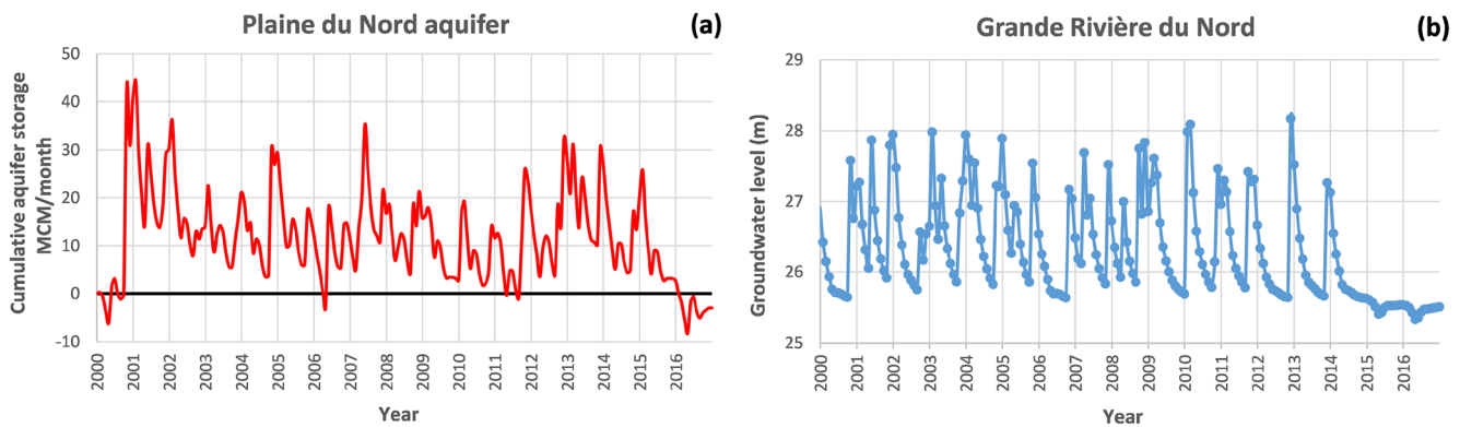
Fig. 14 Transient groundwater dynamics in the Plaine du Nord during the period 2000 to 2016 with a variation of cumulative aquifer storage simulated and b variation of simulated heads in Grande Rivière du Nord
