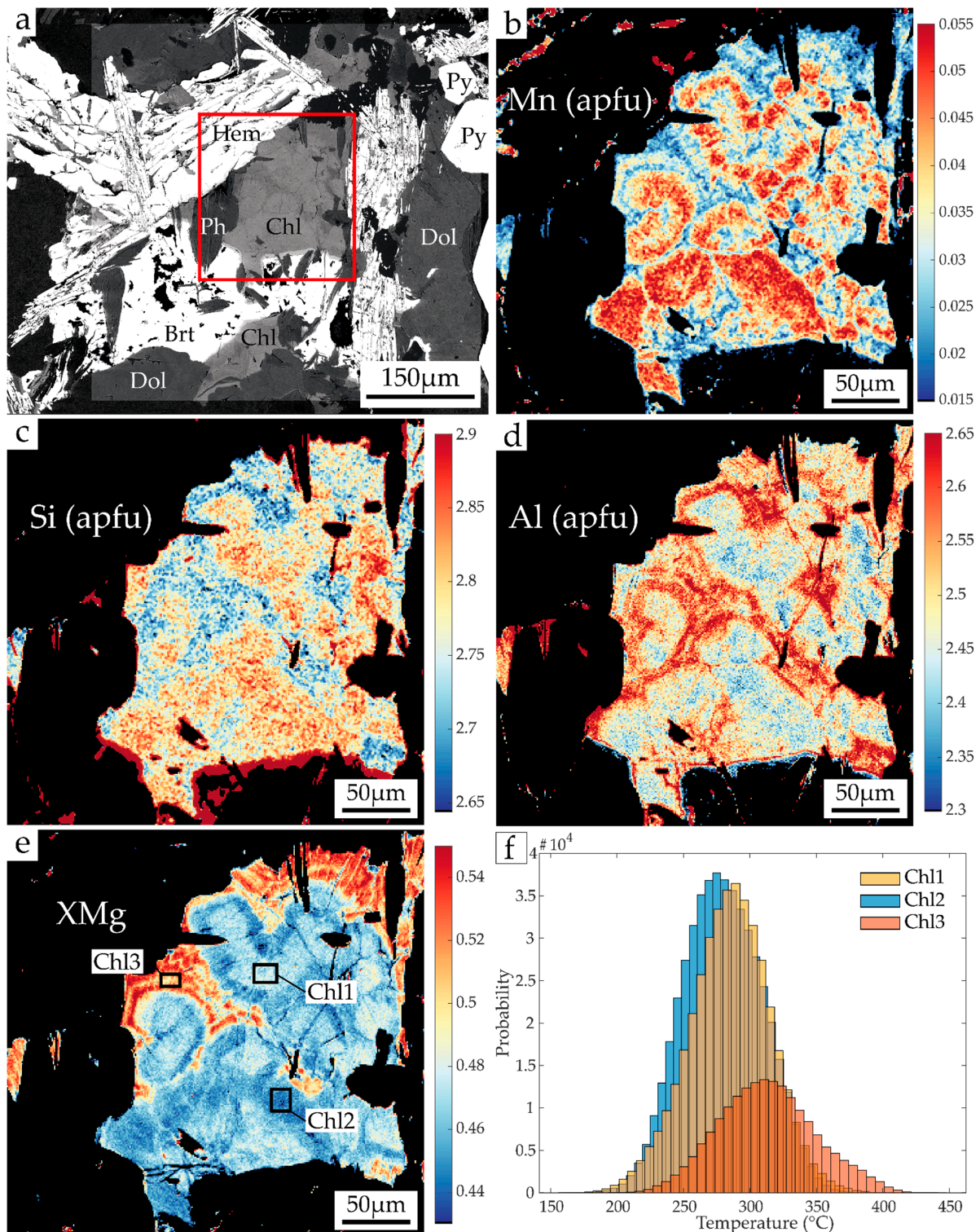
Figure 8. (a) Backscatter (BSE) electron image of euhehal rosette-shaped chlorite aggregates with chemical zoning. The red frame displays the zone of the X-ray map. Quantified X-ray chlorite maps (in apfu) of: (b) Mn; (c) Si; (d) Al; (e) XMg content ( \text{XMg} = \text{Mg}/(\text{Mg} + \text{Fe}_{\text{tot}}) ) with black boxes showing the pixel zone analyzed of each representative chlorite zone, as discussed in the text. (f) Histogram of chlorite temperature formation calculated on each pixel from the map.
