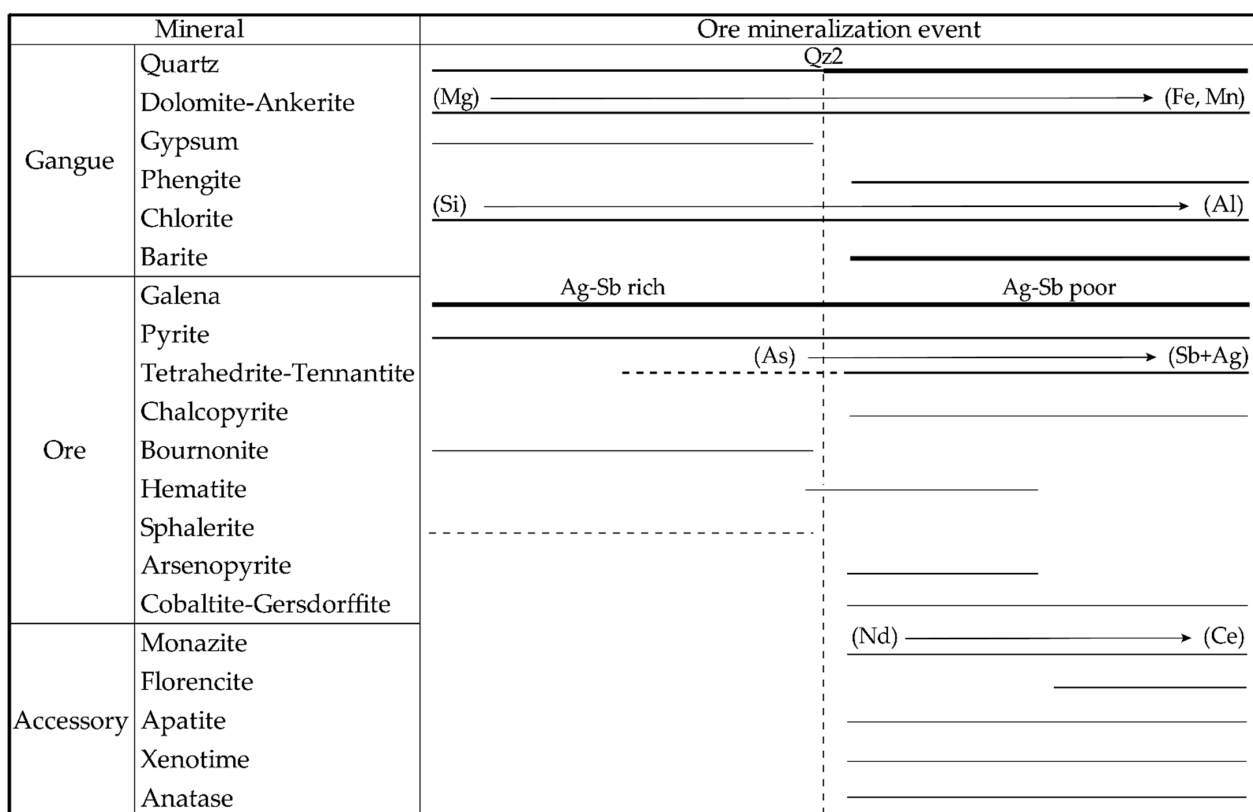
Figure 6. A common paragenesis for the Macôt-la Plagne and the Peisey-Nancroix Pb-Ag deposits. The thickness of the line represents the proportion of each phase.
