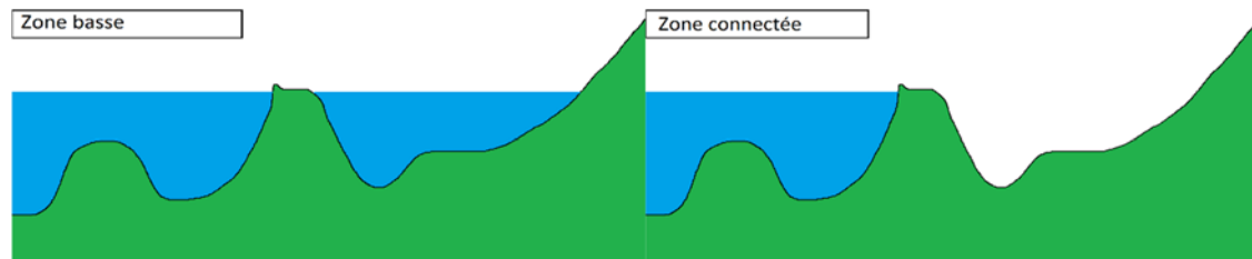
Figure 1. Methods for filling in the flooded areas for a given sea level according to the “Low Zone” on the left and the “Connected Zone” method on the right.
