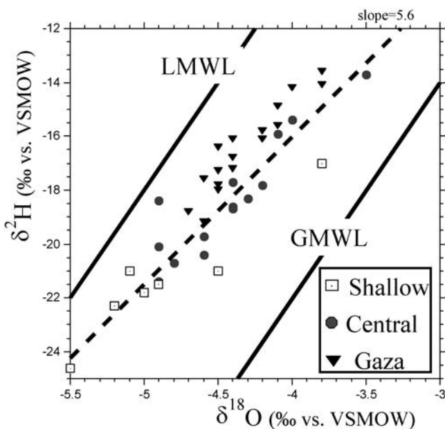
Figure 6. Plots showing δ 2 H versus δ 18 O values (versus SMOW) of groundwater from the coastal aquifer, divided by the different water types. Note the slope of the data point (5.6) relative to the local meteoric water line (LMWL) and global meteoric water line (GMWL).
