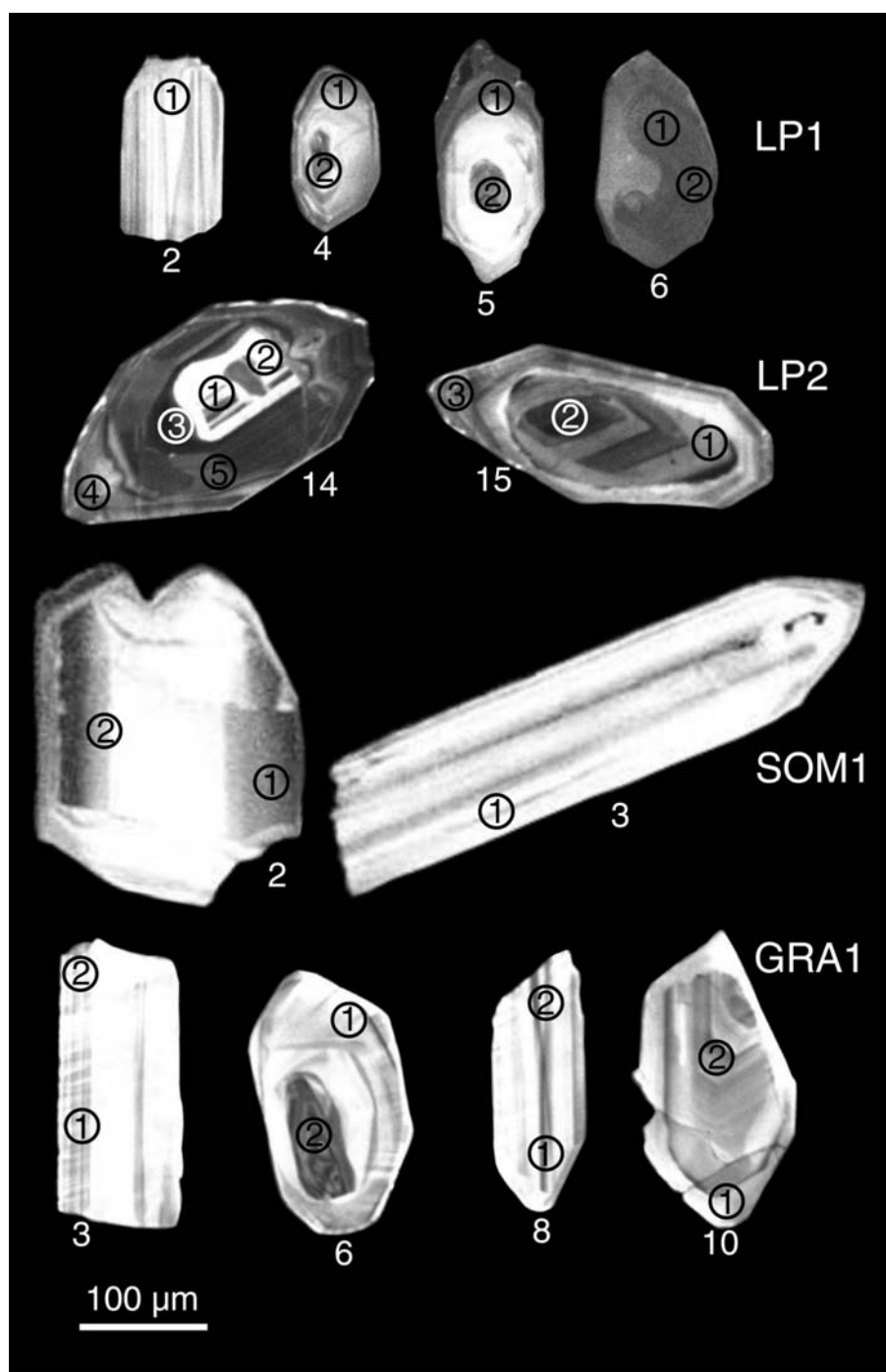
FIG. 4. – Representative cathodoluminescence images of zircon grains analysed using SHRIMP II. Spot size is 20–25 µm. LP 1: grains 2, 4, 5 and 6; LP 2: grains 14 and 15; SOM 1: grains 2 and 3; GRA 1: grains 3, 6, 8 and 10.
