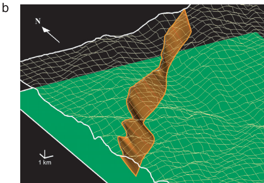
Fig. 4. 3D model of the “accident médian”: a) representation of the data used and b) numerical interpolation of the 3D surface.
