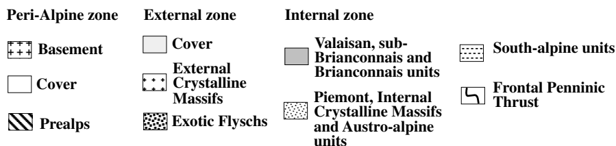
Fig. 1. Location of the study area in the Western Alps (after Debemas & Kerckhove 1980).
