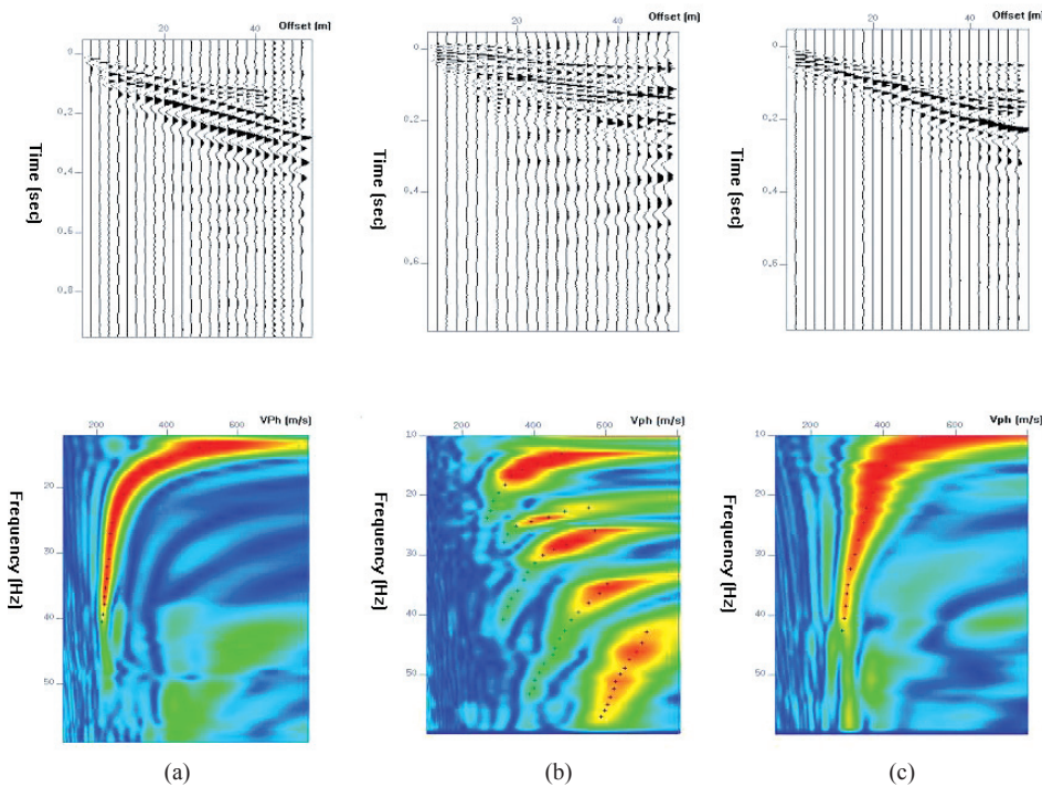
FIGURE 4 MASW shots and the dispersion diagram recorded at the Parc Floral site in (a) the southern, (b) the central and (c) the northern parts of the high-resolution profile.
