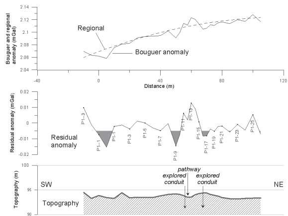
FIGURE 5 Profile 1: Bouguer anomaly, residual anomaly and topography with location of explored conduits and pathway.
