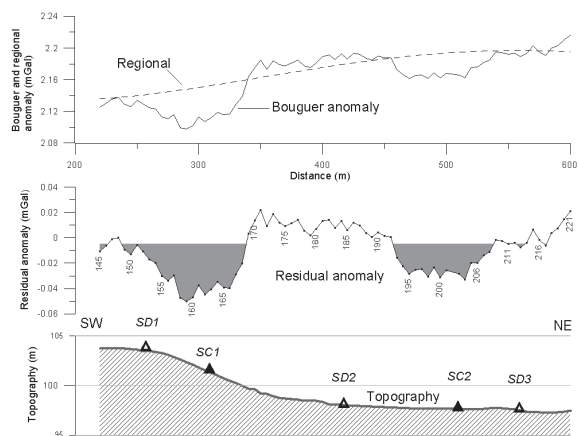
FIGURE 7 Profile 3: Bouguer anomaly, residual anomaly and topography with location of control boreholes.
