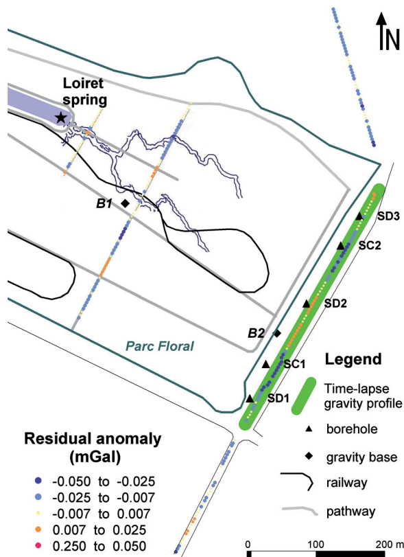
FIGURE 8 Residual gravity anomalies superimposed on the explored karst map, showing the locations of the gravity bases and control boreholes.
