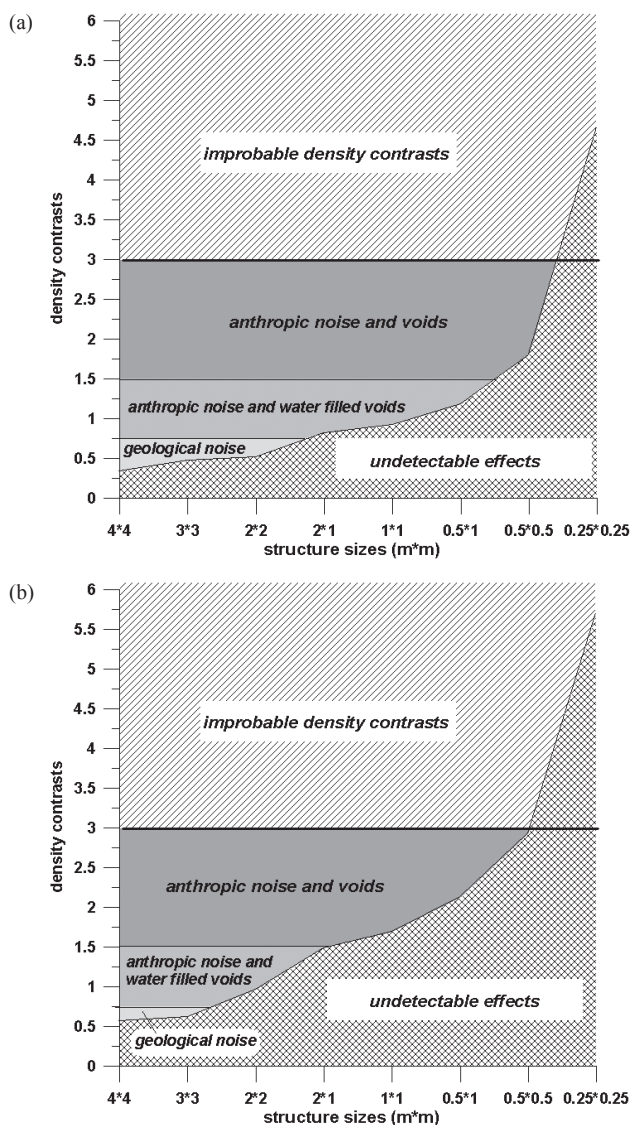
FIGURE 3 Density variations detectable by measurements with (a) 5 \mu\text{Gal} and (b) 10 \mu\text{Gal} uncertainties.
