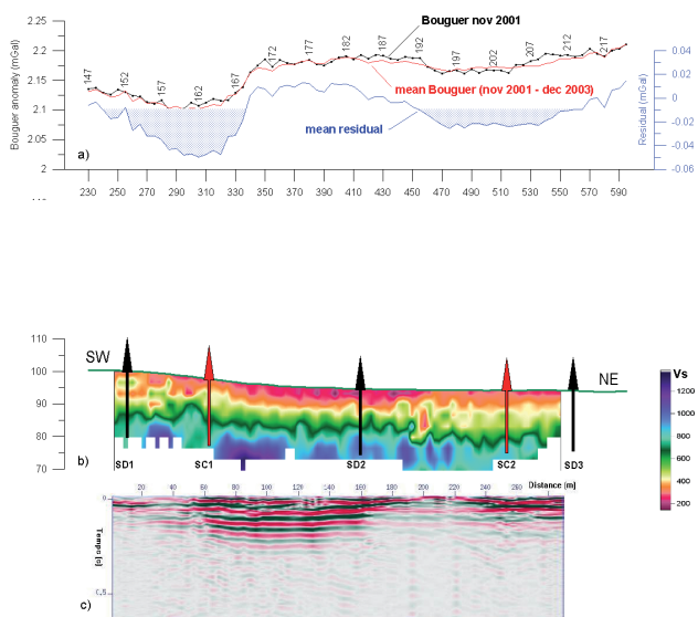
FIGURE 9 High-resolution MASW and microgravity reconnaissance along the central part of Profile 3: (a) gravity anomalies; (b) V_s velocity section; (c) surface-wave image stack.
