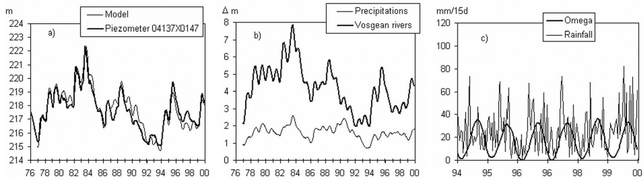
Figure 10. Inverse modeling of groundwater recharge (piezometer 04137X0147 representative of the confined part of the aquifer). (a) Comparison of observed and modeled pressure heads. The Nash coefficient is 0.88. (b) The components of the piezometric variations above the reference level (211.95 m). Contribution of the Rhine is zero. (c) The effective rainfall threshold \Omega(t_i) ; 52.9% of total rainfall contributes to groundwater.
