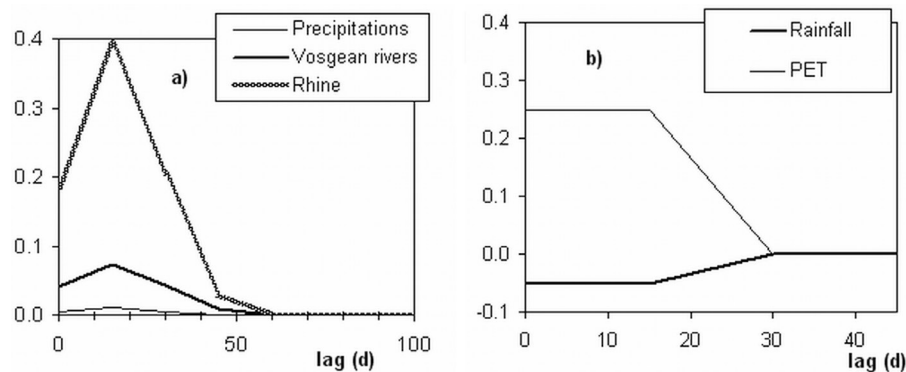
Figure 7. Piezometer 01698X0002. a) Impulse responses \Gamma , \Gamma_1 , \Gamma_2 relative to precipitations and exchanges with Vosgian rivers and Rhine. (b) Impulse responses of the effective rainfall threshold \Omega to rainfall and potential evapotranspiration (PET).
