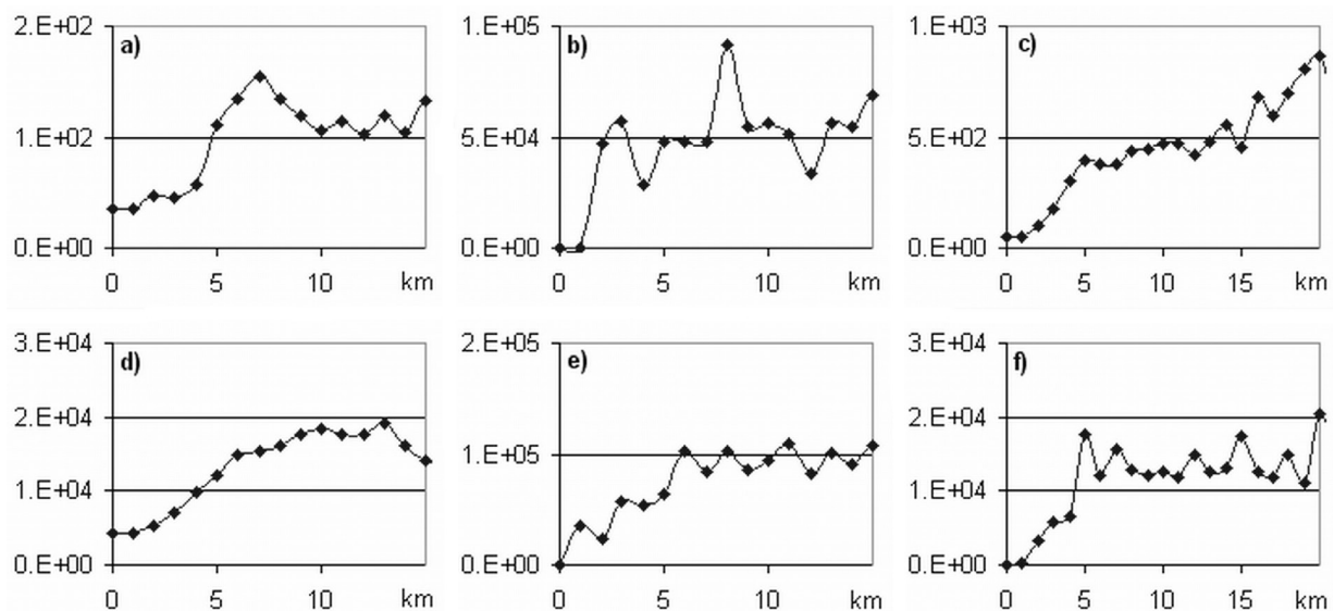
Figure 14. Mean variograms of the contribution to the recharge of (a) the rainfall, (b) the Rhine, and (c) the Vosgian drainages, and mean variograms of the response time of the water table to (d) the rainfall, (e) the Rhine, (f) the Vosgian drainages.
