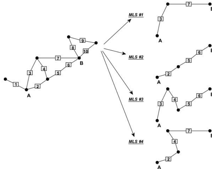
Fig. 2 - Decomposition of the A-B routes into four MLSs, for an illustrative network. Black dots represent intersections in the network, and grey rectangles represent components. The connectivity between A and B constitutes the system performance S .
