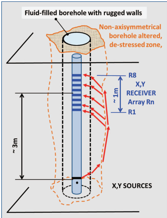
Fig. 16. Dipole Array Sonic tool in the borehole. Two birefringence detection processing routes: A) Alford type, 4x Rn response signal detection between source and mid array positions ( \sim 3 m). B) Azimuthal slowness measurement scan over the Rn array interval only ( \sim 1 m), independently for the azimuths of linearly polarized VS-fast and VS-slow principal shear modes.
