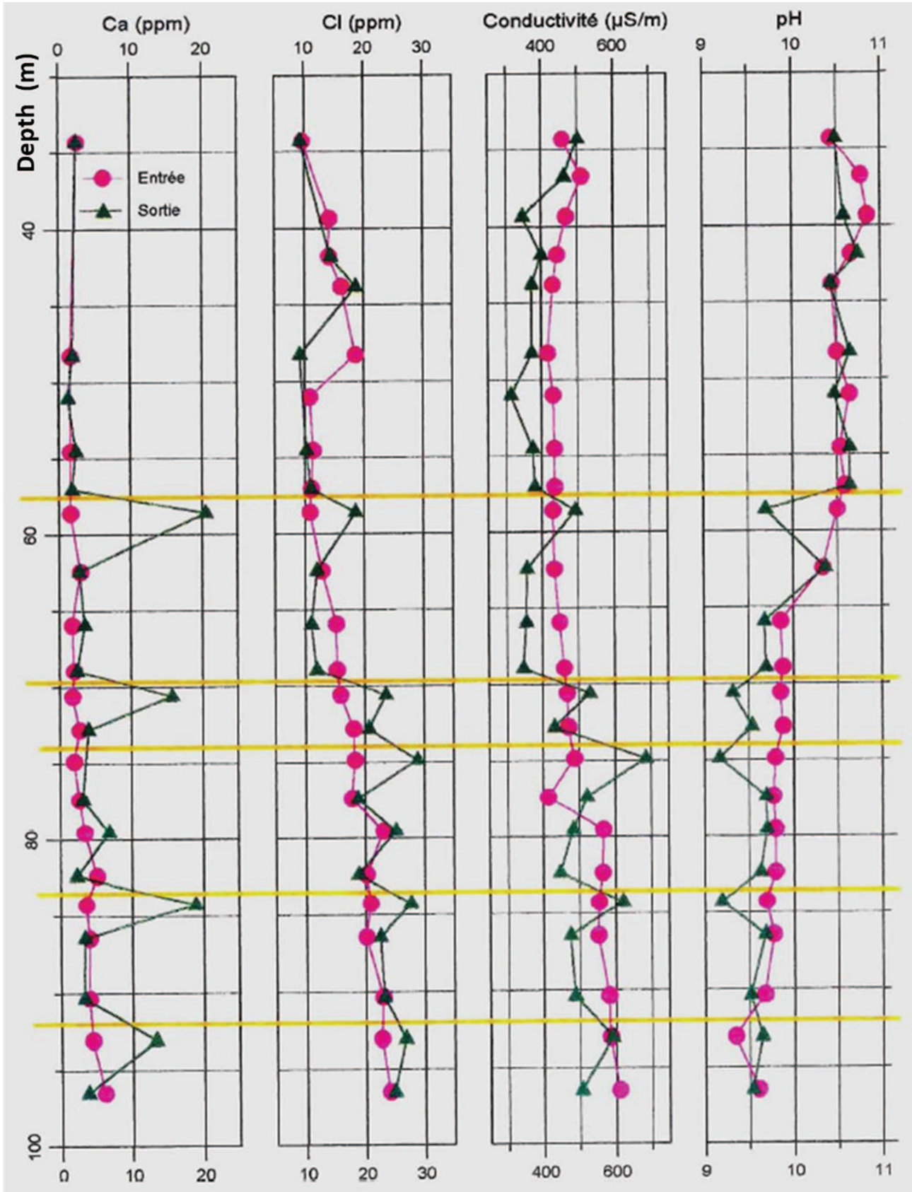
Fig. 6. GPF-Ardèche, MM1 borehole, geochemical results from Mud logging while drilling. The yellow bars indicate depths of confirmed permeability.
