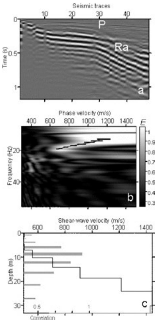
FIGURE 2 (a) Example of a seismic shot recorded on the Super-Sauze site, showing the P-waves (P) as first arrivals and Rayleigh waves (Ra) strongly affected by lateral velocity variations. (b) The corresponding dispersion image with the estimated dispersion curve (black line). This plot represents the normalized energy distributions E (equation (2)) of Rayleigh wave propagation modes. (c) Inverted shear-wave velocity profile. The correlation of inverted parameters, giving the reliability of velocities, is plotted in grey.
