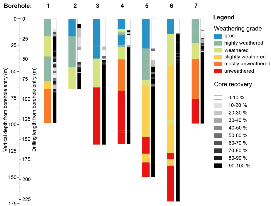
Figure 3. Geological boreholes drilled by the Commissariat à l'Énergie Atomique, showing the granite weathering grade and the core recovery percentage. The borehole locations are shown in Fig. 1. The “highly weathered” and “weathered” layers were interpreted as corresponding to the fissured layer, while the “slightly weathered” to “unweathered” layers were interpreted as corresponding to the bedrock.
