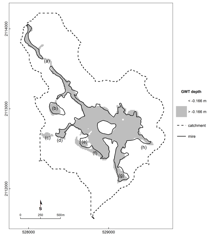
Figure 7. Observed mire boundary based on botanical (Durepaire and Guerbaa, 2008) and pedological (Duranel, 2015) criteria and the predicted mire distribution based on model results (simulated 2001–2013 mean groundwater table depth higher than 0.166 m below ground level). (a–h) refer to locations discussed in the text (see Sect. 3.1).
