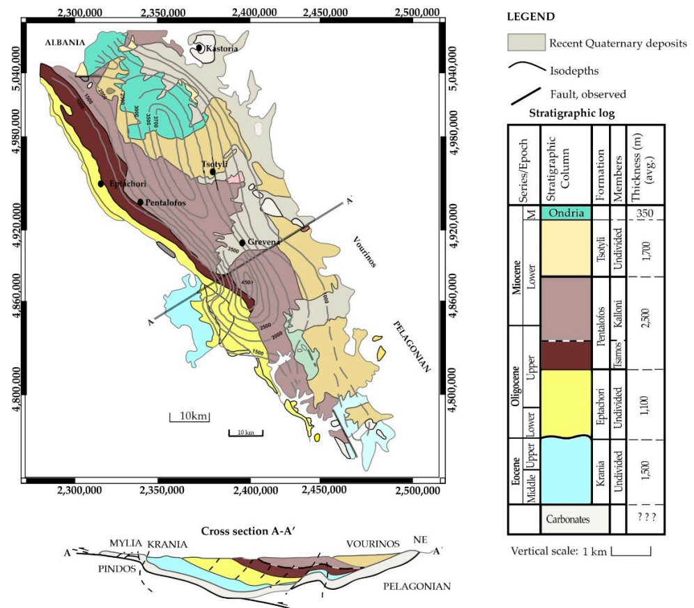
Figure 4. Geological Map and stratigraphic column adapted from Ferriere et al., 2004, of the proposed CO 2 Storage basins in Grevena area depicting Pentalofos and Eptachori formations, scale 1:1,000,000. Cross-sections of the Mesohellenic Trough. Lithological formations: Krania Turbidites, Eptachori, Taliaros, Pentalofos, Tsotyli. M stands for Middle Miocene, scale 1:500,000.
