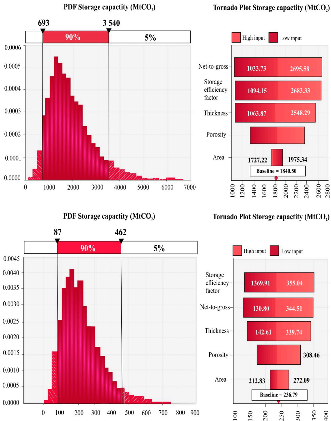
Figure 5. Histograms of storage capacity for the Pentafolos (top) and Epatchori Fm (bottom), resulting from 5000 Monte Carlo runs of Equation (1) using the probability density distributions (PDF's) of parameters in Tables 7 and 8, and the corresponding Tornado plots for each geological formation.
