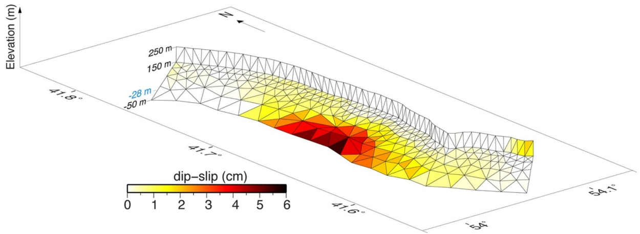
Figure 5. 3D view with 1:8 vertical exaggeration of the modelled near flat décollement (~2°) connected to the steeper scarp (60°) at the crown of the landslide with the best-guess slip distribution. The - 28 m value shown in blue on the vertical axis indicates the water level. Figure generated using Generic Mapping Tools (GMT v5.3.1; http://gmt.soest.hawaii.edu/ ).
