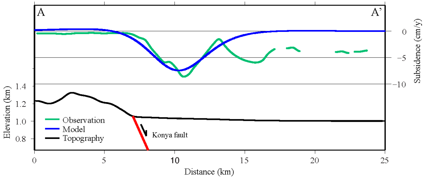
Figure 15. Profiles showing modeled (blue) and observed (green) subsidence due to potential slow slip on the Konya fault.
