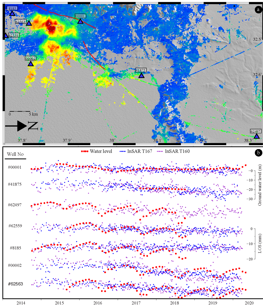
Figure 13. Correlation between subsidence and groundwater level change. (a) Location of available wells in the study area shown on the n LOS velocity field on T160. (b) Time series of InSAR together with piezometric measurements in the wells shown in (a).
