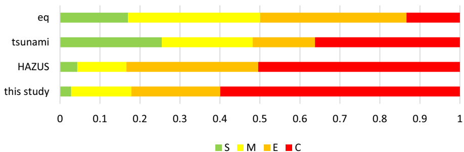
Fig. 28 Damage probabilities for the IOM event in Guadeloupe, Pointe-a-Pitre (PàP) for Slight (S), Moderate (M), Extensive (E) and Complete (C) damage states resulting from (i) earthquake event, (ii) tsunami event, (iii) HAZUS approach for combining the damages coming from earthquake and tsunami and (iv) this study approach for combining the damages coming from earthquake and tsunami
