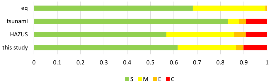
Fig. 27 Damage probabilities for the IOG event in Trinité for Slight (S), Moderate (M), Extensive (E) and Complete (C) damage states resulting from (i) earthquake event, (ii) tsunami event, (iii) HAZUS approach for combining the damages coming from earthquake and tsunami and (iv) this study approach for combining the damages coming from earthquake and tsunami
