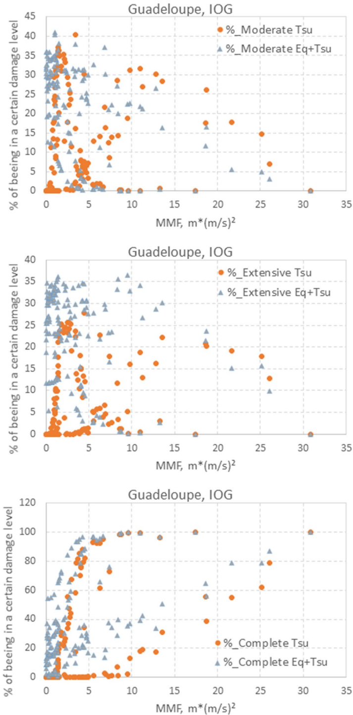
Fig. 25 Relation between the moment flux ( H^*v^2 ) and the Damage States (Moderate, Extensive, and Complete) calculated for tsunami event and for combined tsunami and earthquake events, for Guadeloupe Island
