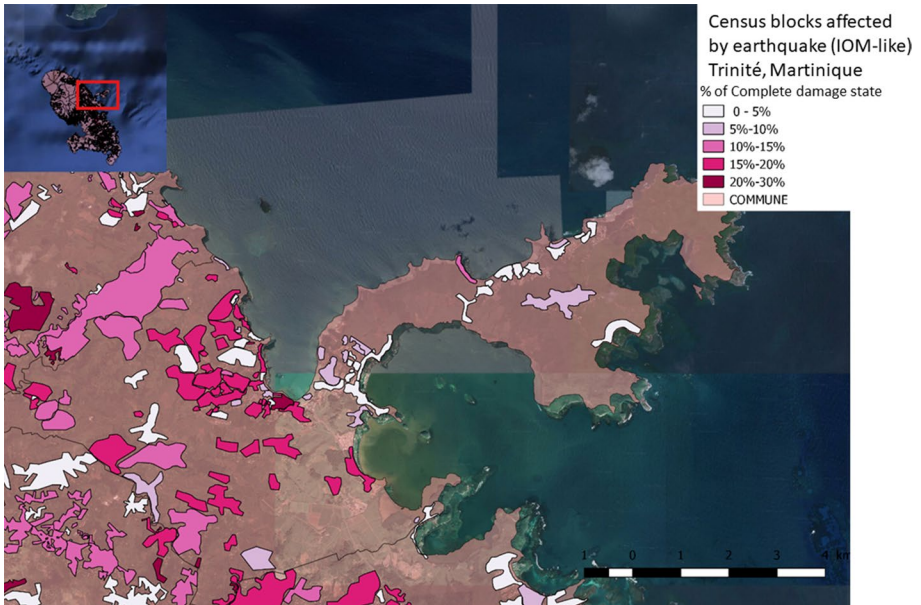
Fig. 19 Martinique IOM-like (inspired from 1839 earthquake) earthquake damage, zoom on Trinité: percentage of complete damage state per census block
