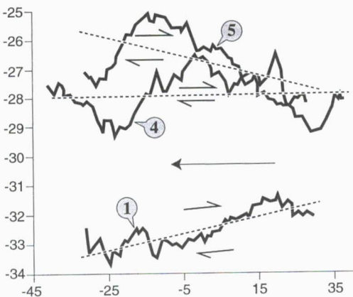
Figure 2. Profiles No 1, 4, and 5 of the lower wall (direction 0°) with their local regression lines in the vertical plane in which σ n and shear direction (arrow) are located. Units on the axis are mm.
