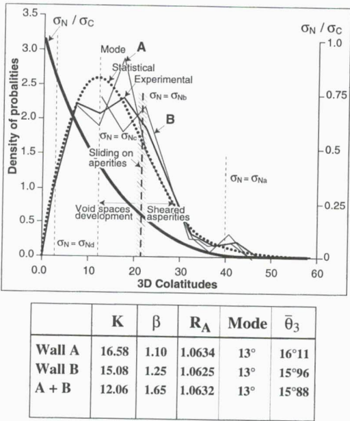
Figure 4. 3D reconstructed distributions and models for colatitudes \theta_3 with characteristics of the fitted models for 3D distribution.
