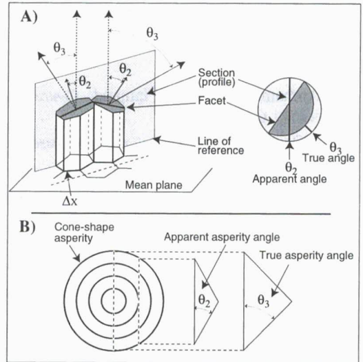
Figure 1. A) Definitions of \theta_2 and \theta_3 and stereographic projection showing the dependance of \theta_2 on \theta_3 the direction of the vertical section plane (From Riss & Gentier, 1989). B) Illustration of the bias 2d apparent asperity angle \theta_2 relatively to the true asperity angle given by \theta_3 .
