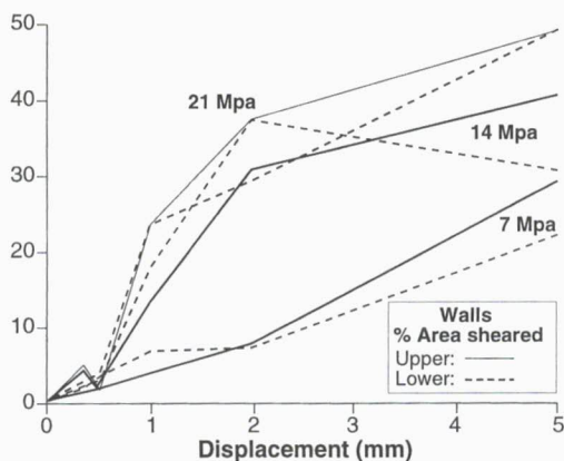
Figure 6. Proportion of damaged area evaluated on upper and lower joint walls for \sigma_N = 7, 14, 21 MPa in relation with shear displacement.
