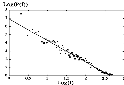
Fig. 4. The power spectrum P(f) of the profile as a function of the frequency f in a log-log diagram. A linear regression of slope 2.60 is shown. The corresponding value of the roughness exponent is 0.80.
